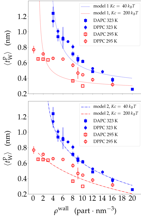
Figure 8: Equilibrium confined water thickness \langle t_W^p \rangle as a function of wall density \rho^{\text{wall}} , for the SLB simulations of two lipids at two temperatures. Top : The lines correspond to fits using Eq. 5 with 4 parameters. Bottom : The lines correspond to fits using Eq. S16, emerging from Eq. 7 with 6 parameters. Two of these parameters are the bending moduli K_c , fixed at 40 k_B T and 200 k_B T for the fluid and gel phases respectively 58–61 .
