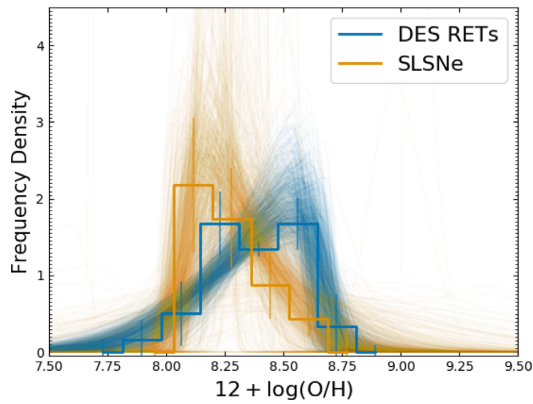
Figure C5. Results of the MCMC fits to the PDFs of metallicity for DES RETs and SLSNe, accounting for uncertainties in each bin.
