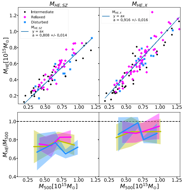
Figure 6. First row: The HE masses M_{HE,SZ} and M_{HE,X} as a function of M_{500} for the AGN simulations at z=0 using the analytical fitting method. Only clusters with reliable fits are shown. A linear fit is performed and the value of the slopes are listed in the plots. The relaxed clusters are represented as magenta diamonds, the disturbed ones as blue squares, and the intermediate as black circles. Second row: A binned average of the ratio of M_{HE} (the same of the first row) and M_{500} is represented as a function of M_{500} . The magenta and blue lines are the averages of the relaxed and disturbed clusters, respectively, while the yellow one the average over all the clusters. The shaded regions show the 1\sigma intervals.
