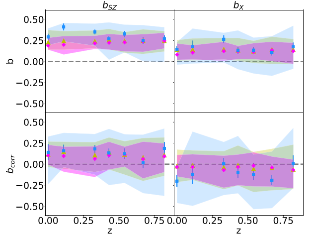
Figure 9. The redshift evolution of the biases, b_{\text{SZ}} (left-hand panels) and b_X (right-hand panels), from the AGN simulations. The reliable fits have been used to compute them. The median values of the bias for all clusters, relaxed, and disturbed are represented with yellow triangles, magenta diamonds, and blue squares, respectively. The error bars correspond to bootstrap errors. The shaded regions represent the 16th and 84th percentiles. In the bottom panels, the corrected bias factors b_{\text{corr}} (see Section 6.4) are also plotted.
