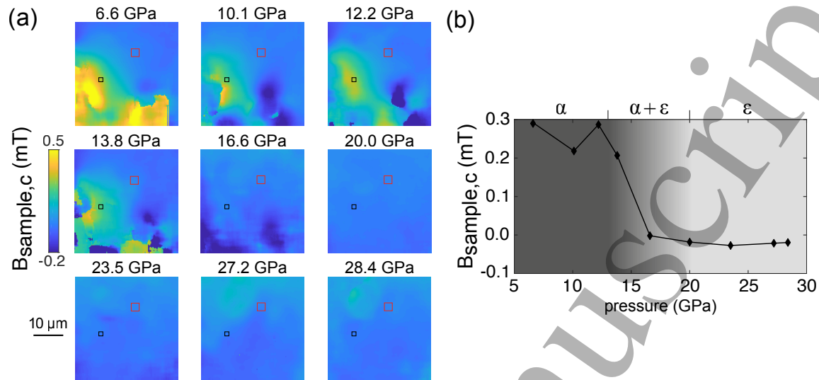
Figure 4. (a) Color maps of the magnetic field projection B_{\text{sample},c} of the magnetic field created by the iron magnetization along the c axis of the selected NV family. As the pressure increases, the local positive and negative variations of B_{\text{sample},c} progressively disappear, until the sample no longer exhibits any magnetic properties. Red squares ( 7 \times 7 pixels) indicate the chosen reference area to extract sample magnetization effects from pressure and bias field ones. Black squares ( 11 \times 11 pixels) indicate the area over the sample where signal is averaged for figure 2b. (b) Measurement of B_{\text{sample},c} averaged over the black square shown in panel (a) as the pressure in the DAC chamber increases. A greyscale pattern is overlaid to indicate the start and the end of the \alpha -Fe to \epsilon -Fe structural transition independently determined using the XRD pattern. The evolution of the magnetic field created by the iron magnetization is consistent with the XRD data.
