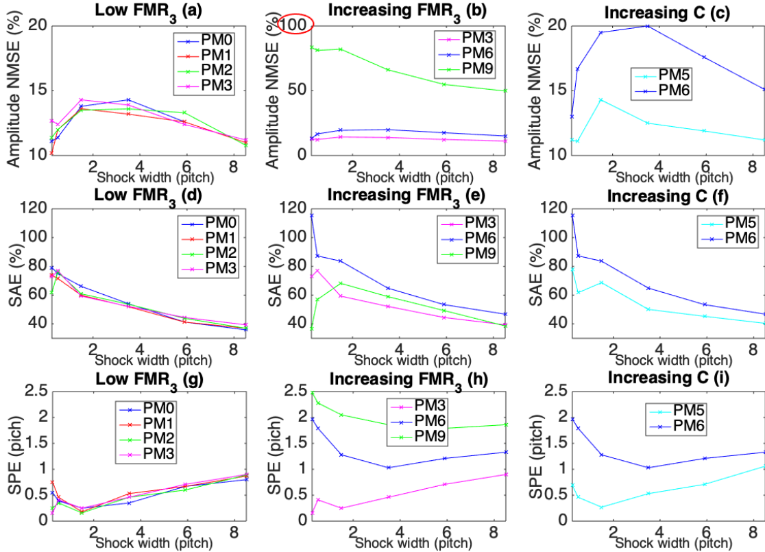
Fig. 9. NMSE, SAE and SPE values for different shock widths and phase modulations.
