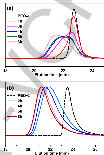
Figure 1. HT-SEC traces of the polymers resulting from ethylene polymerization in the presence of PEO-1 (a) and PEO-2 (b) at 80 °C and 80 bar.
