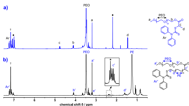
Figure 2. ^1\text{H-NMR} spectra of PEO-2 (a) and after 4 hours of block copolymerization with ethylene (b), corresponding to entry 11 of Table S1. (†) NMR residual solvent benzene, (●) toluene collecting solvent.
