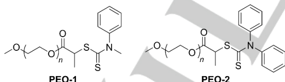
Scheme 1. Chemical structures of PEO-1 and PEO-2 dithiocarbamates.
