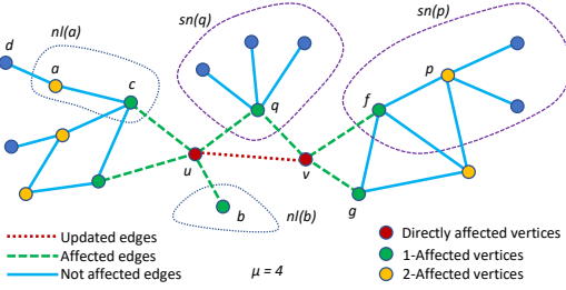
Fig. 5. Affected vertices, edges, super-nodes and noises w.r.t. a changed edge (u, v) \in U
