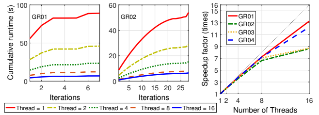
Fig. 12. Cumulative runtimes of anySCAN after each iteration of its anytime scheme for different numbers of threads (left) and the final runtime scalability (right)
