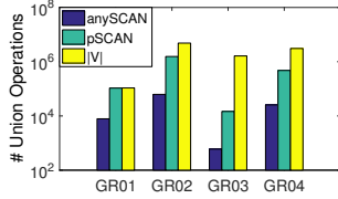
Fig. 14. Number of performed Union operations for GR01 to GR04
