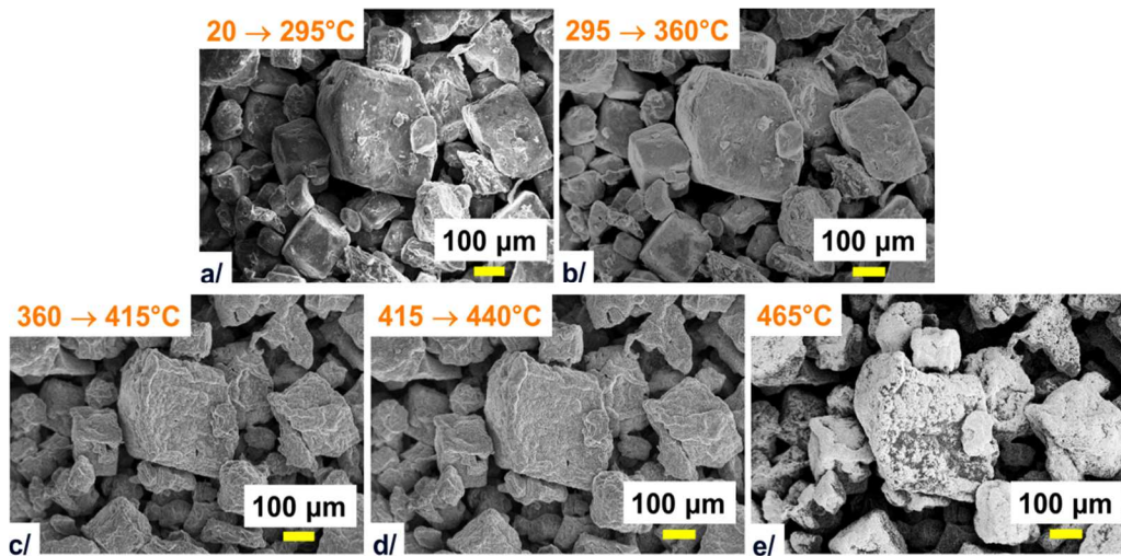
Fig. 2. a/ Thermally-induced transitions of LiOH powder during the heating step under secondary vacuum with b/-d/ a highlight of the intermediate surface of LiOH, and e/ at the beginning of the surface conversion into Li 2 O.
