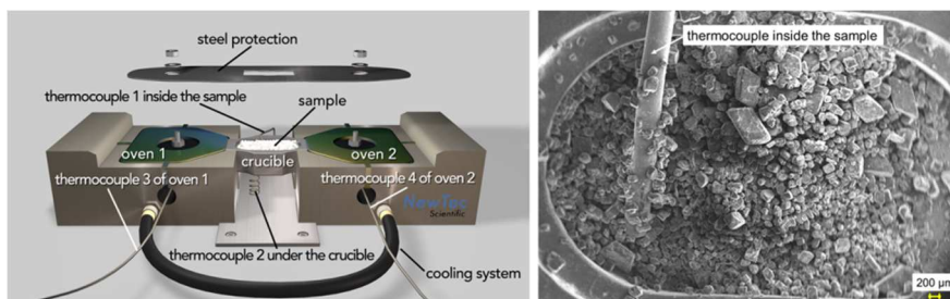
Fig. 1. On the left, the hot stage used for the HT-SEM experiments made up of two ovens allowing applying either a homogeneous working temperature or a temperature gradient. A protection is added to avoid, as possible, the heat loss and the SEM chamber contamination, without avoiding the sample visual monitoring. On the right, top view of LiOH powder inside the HT-SEM stainless steel crucible.
