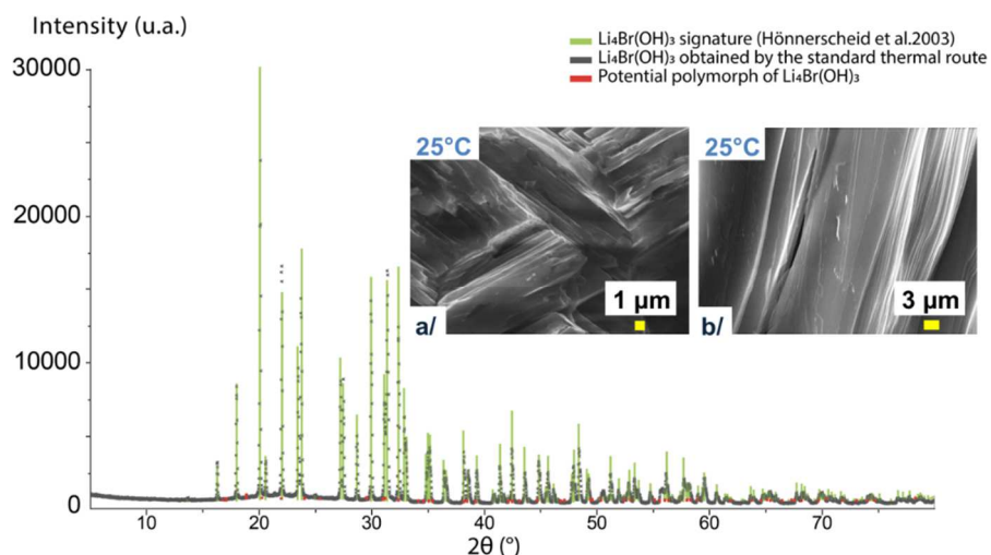
Fig. 11. XRD diffractogram of the 3\text{LiOH} \cdot \text{LiBr} mixture after the thermal treatment inside the SEM chamber under low pressure condition confirming the \text{Li}_4\text{Br}(\text{OH})_3 obtention as described by [23] with its related morphology.
