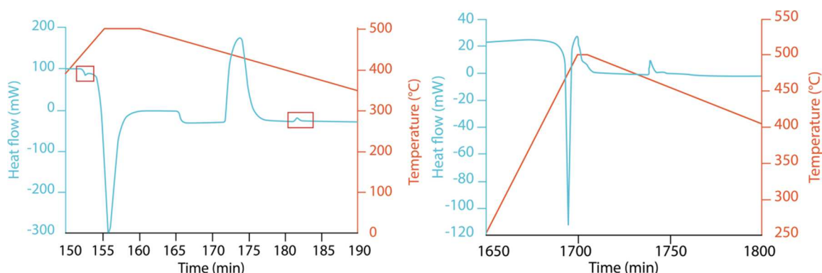
Fig. 4. LiOH underwent 6 thermal cycles: Here on the left, third LiOH thermogram obtained at a heating scanning rate of 0.3 °C/s. The red frames show the LiOH softening. On the right, the third thermogram obtained for a heating scanning rate of 0.1 °C/s. The same palier of 5 min at 500°C has been applied for both protocols.
