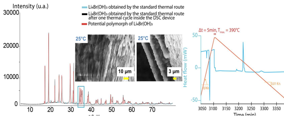
Fig. 12. XRD diffractogram with the related morphology of the potential \text{Li}_4\text{Br}(\text{OH})_3 polymorph obtained with the Alfa Aesar educts. On the right, its related DSC signal.
