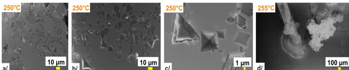
Fig. 10. a/-c/ Occurrence of the LiOH-primary solid phase in the liquid mixture, followed by d/ the dissolution of the LiOH prisms into the liquid mixture.
