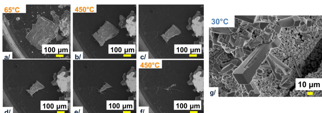
Fig. 6. a/-f/ Highlight on the LiBr grain sublimation at 450°C and g/related LiBr crystallisation on the edge of the stainless steel protection above the crucible.
