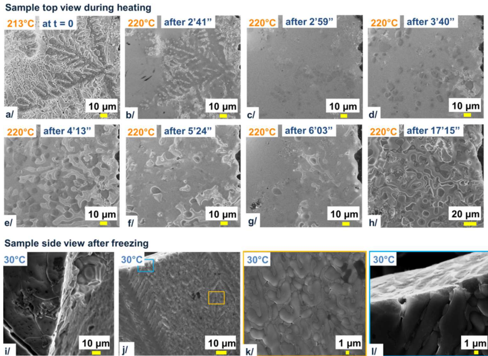
Fig. 9. a/-h/View from the sample top held at 220°C because of the rapidity of the observed phenomenon: Example of the oscillatory motion effect due to the reaction and infiltration of the LiBr-rich liquid with the LiOH evolving structure once it has been fully covered during the heating step, i/-l/ View from the sample side during another similar experiment fastly cooled up to 30°C.
