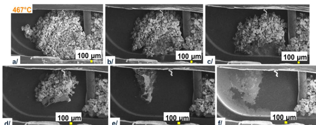
Fig. 5. Thermally-induced transitions of ground LiBr under secondary vacuum during the heating step maintained at 467°C.
