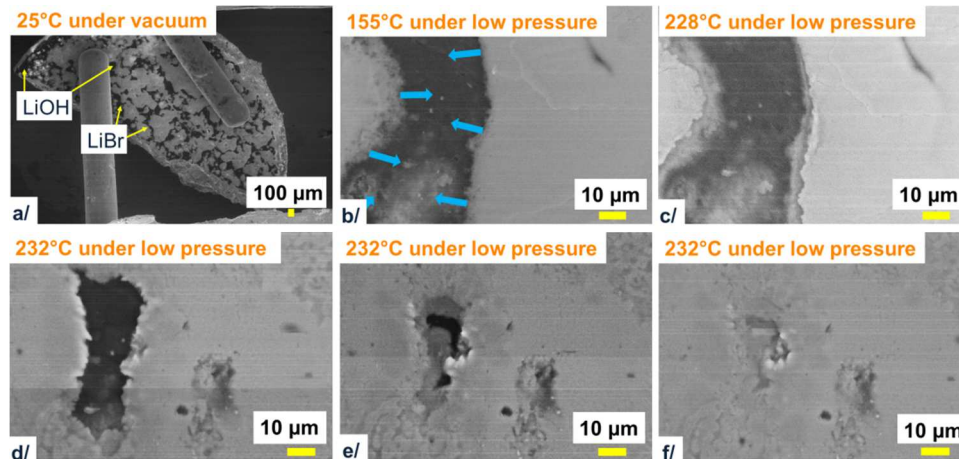
Fig. 8. a/ Pellet of 3\text{LiOH}\cdot\text{LiBr} where \text{LiBr} corresponds to the white areas and \text{LiOH} to the dark ones. b/-f/ Zoom in on the \text{LiBr}/\text{LiOH}/\text{LiBr} interfaces and layer-by-layer covering process visualisation (blue arrows).
