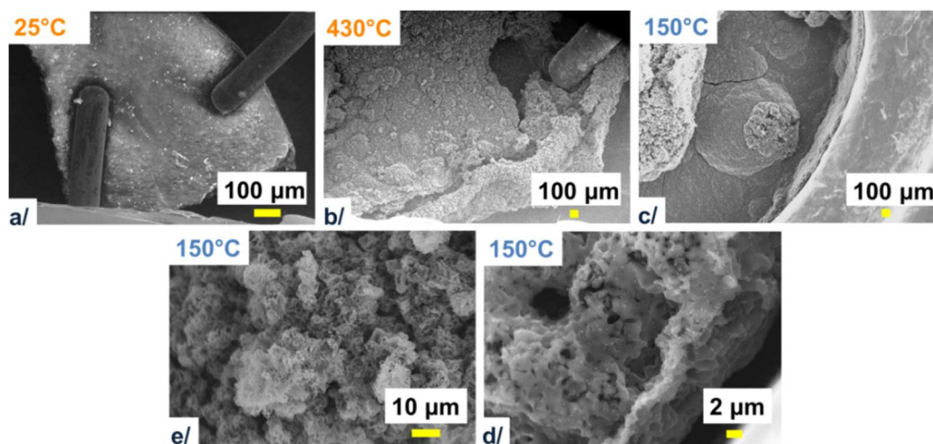
Fig. 3. a/-c/ Highlight on the LiOH melting during the heating step and after cooling at a partial pressure of 10 Pa. e/-d/ Zoom in on the sample at the edge of the crucible.
