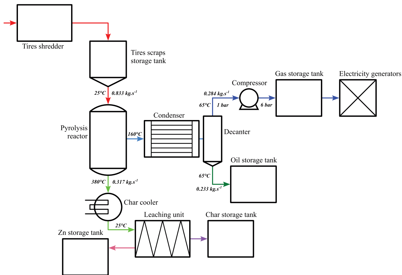
Fig. 2. Simplified flowsheet of the ELT pyrolysis process.
