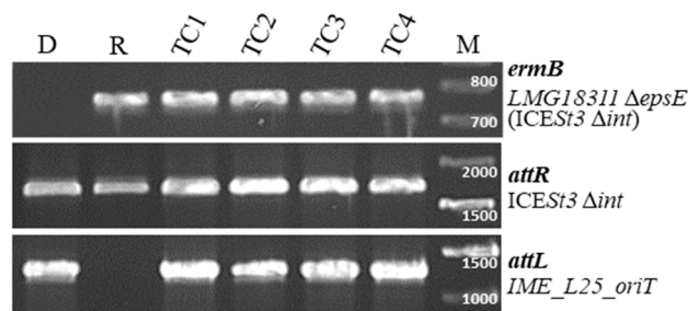
Figure 4. PCR analysis of four transconjugants (TC1 to TC4) obtained using the mating pair LMG18311(ICEST3 \Delta int::IME_SsallL25_oriT) (donor D)/LMG18311 \Delta epsE (ICESt3 \Delta int) (recipient R). Specific regions were amplified to discriminate the recipient strain, ermB for \Delta epsE, and attL for IME_SsallL25_oriT. The integrase deletion (done by insertion of a chloramphenicol resistance cassette) was detected with the amplification of the attR site of ICESt3. The sizes of the PCR fragments were confirmed by parallel migration of a DNA ladder (M for marker on the figure). The primers pairs used for these amplifications and expected sequence lengths are listed in Table S1.
