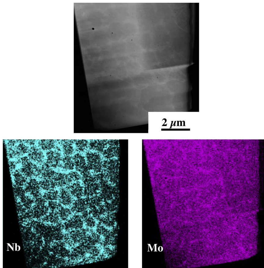
Fig. 4. HAADF-STEM image and relative X-ray maps of the microstructure of the LBM alloy. The results show that Nb(L c ) and Mo(L c ) segregations are responsible for the cellular microstructure observed in Fig. 3.
