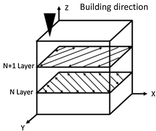
Fig. 1. Schematic description of the 3D building strategy.
