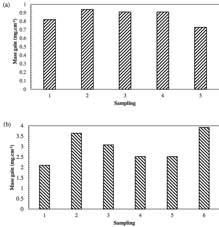
Fig. 5. Mass gains of the as-manufactured LBM-Inconel 625 after isothermal oxidation in still lab air with exposures of a) 400 h at 900 °C and for b) 50 h at 1050 °C.
