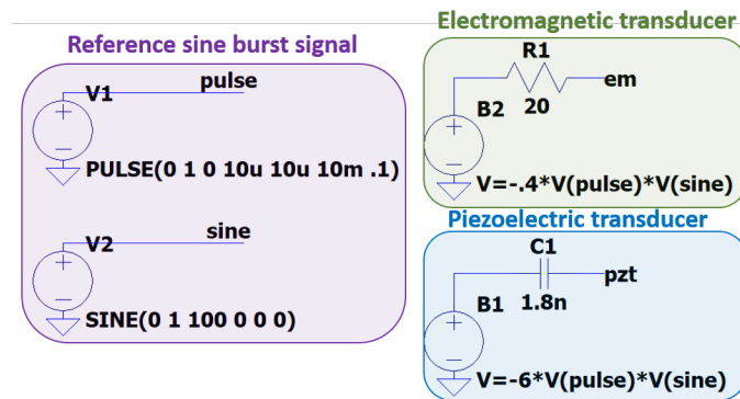
(a) Transducer models
