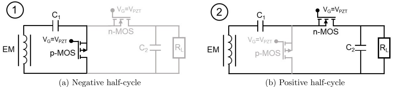
Figure 4: Circuit operations
