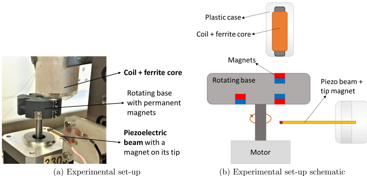
Figure 9: Experimental set-up
