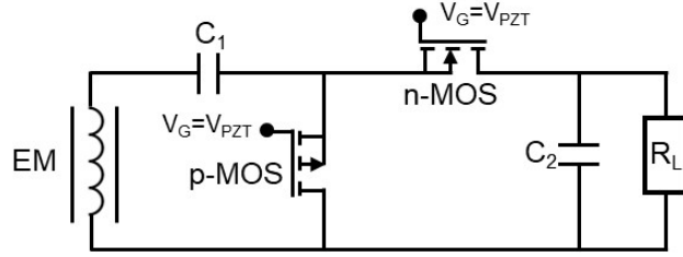
Figure 3: Circuit schematic
