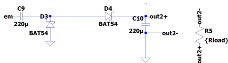
(c) Schottky diodes interface
