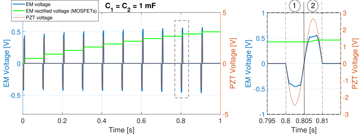
Figure 5: Simulated voltage waveforms (the value of capacitance has been chosen in order to enhance the charge of the capacitors for each cycle); ①: Negative half-cycle; ②: Positive half-cycle
