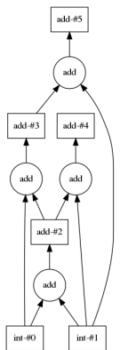
Figure 4: Example of Dask use (left) and relations between Dask delayed objects (right).
