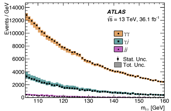
Figure 7: Event yields as a function of the invariant mass of the diphoton pair for the three non-resonant background contributions in the range between 105 and 160 GeV [5].
