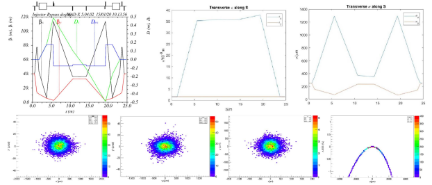
Figure 11: Beam optics (top) and phase space (bottom) of 10° dogleg bypass
