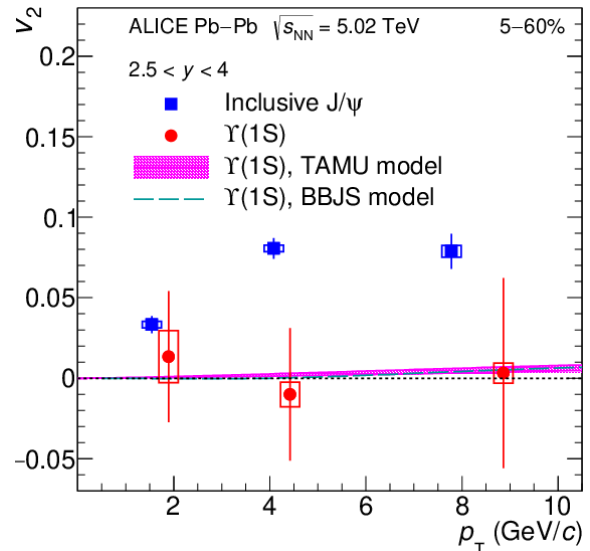
Figure 3: \Upsilon(1S) as function of transverse momentum p_T for centrality class 5–60% and comparison to inclusive v_2(J/\psi) from published 2015 data. The p_T ranges correspond to 0–3, 3–6, 6–15 GeV/c. The major contributions for the TAMU model [17] corresponds to \Upsilon(1S) generated by path length dependent suppression and the regeneration. The BBJs model [20] use a 3+1D quasi particle anisotropic escape mechanism based on a hydro-dynamical description with no recombination.
