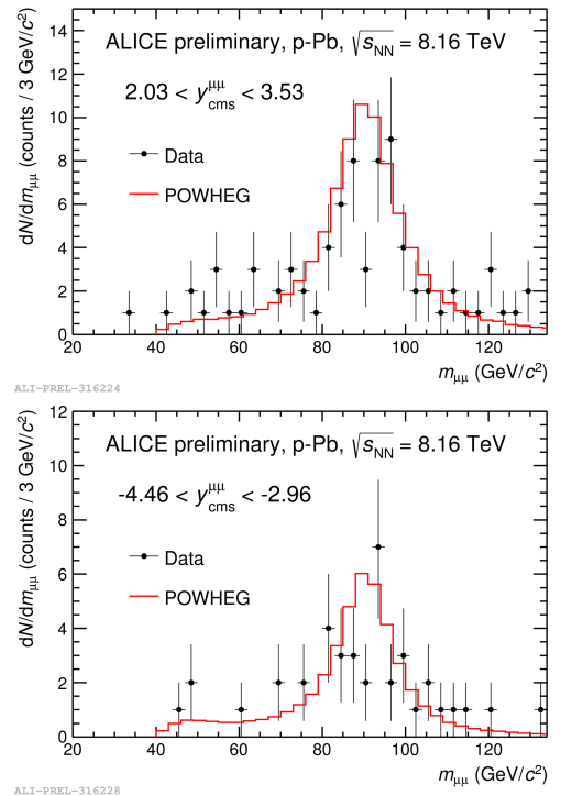
Figure 1: Invariant mass distribution of \mu^+\mu^- pairs for p-Pb collisions at \sqrt{s_{\text{NN}}} = 8.16 TeV for the p-going (top panel) and Pb-going (bottom panel) data samples. The distributions are obtained from muons with -4 < \eta < -2.5 and p_T > 20 GeV/c (black points) and compared to POWHEG simulations (red curve).
