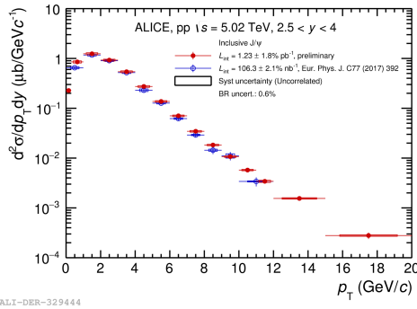
Figure 3: Inclusive J/\psi differential cross section as a function of p_T at forward rapidity in pp collisions at \sqrt{s_{NN}} = 5.02 TeV. The new measurement with 2017 data is shown (red) and compared to the published results of 2015 (blue).
