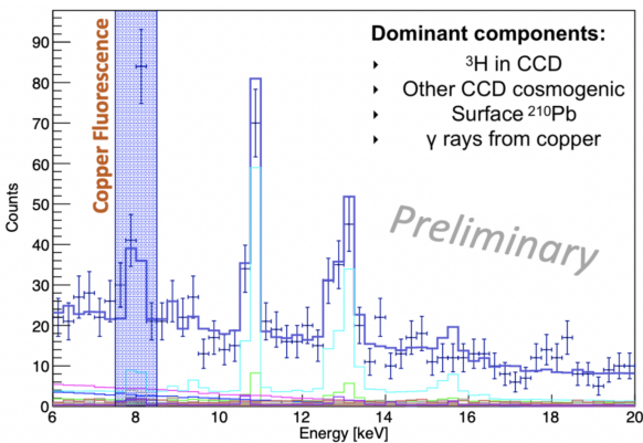
Figure 4: 2-D fit to data projected onto energy.
