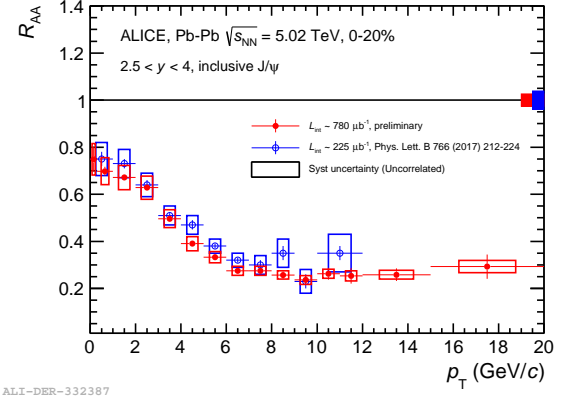
Figure 4: Inclusive J/\psi nuclear modification factor as a function of p_T in most central collisions at forward rapidity in Pb-Pb collisions at \sqrt{s_{NN}} = 5.02 TeV. The new measurement with 2015 and 2018 data is shown (red) and compares to the previous published results (blue).
