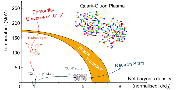
Figure 1: Phase diagram of quantum chromodynamics (QCD) matter. Figure from [6].
