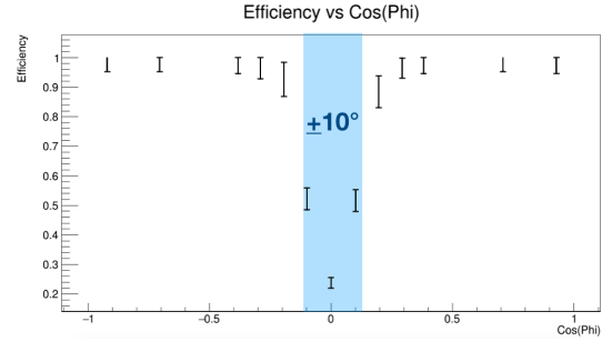
Figure 4: Reconstruction efficiency as a function of the horizontal angle. The efficiency drops drastically when muons are travelling \pm 10^\circ from parallel to a view (when \text{Cos}(\Phi)=0 ).
