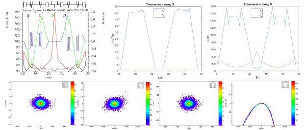
Figure 12: Beam optics (top) and phase space (bottom) of 10° chicane bypass
