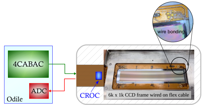
Figure 1: Setup schematic analogous to DAMIC-M
