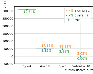
Figure 6: Collision event selection efficiencies of a four top quark MC sample after a loose pre-selection. The last bin corresponds to the selection used in the four top system reconstruction study
