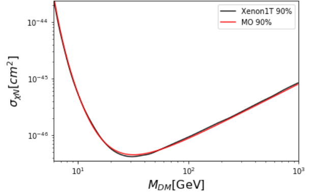
Figure 2: The 90% exclusion cross section for SI interaction by Xenon-1T (black) compared with the 90% exclusion obtained with p_{eff} using micrOMEGAs (red). Note that M_{DM} \equiv M_\chi .
