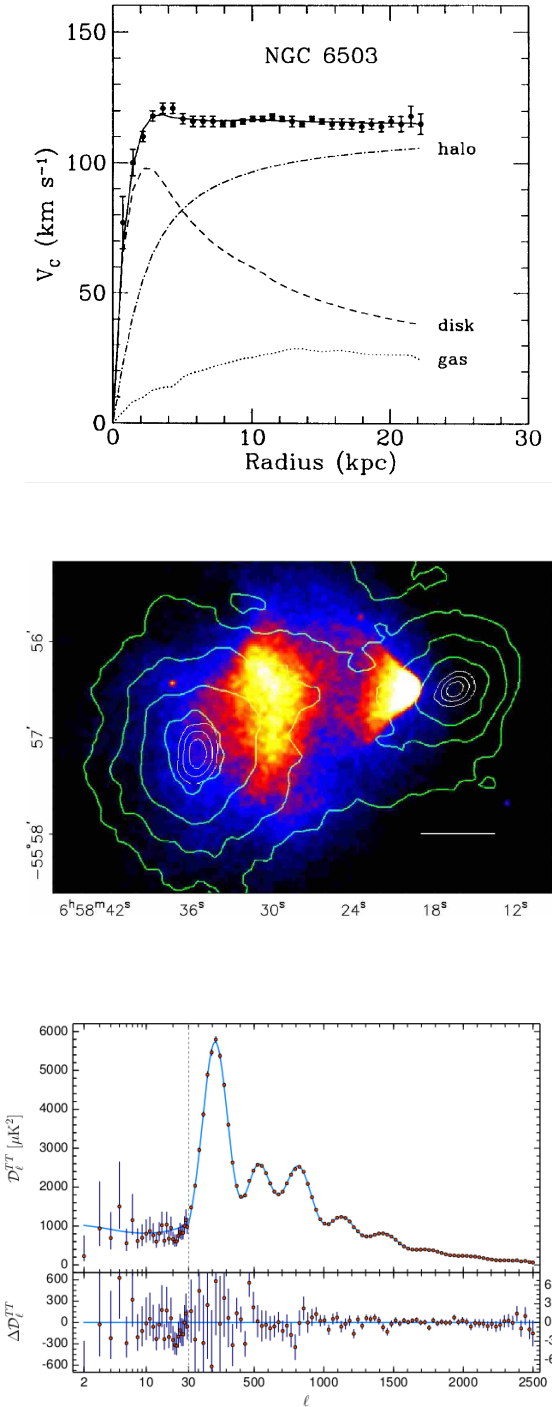
Figure 1: Evidence for dark matter. Top panel: the rotation curve of NGC 6503, taken from [3]. Middle panel: the bullet cluster, taken from [4]. Bottom panel: the CMB temperature power spectrum, taken from [5]. For explanations see text.
