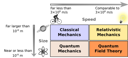
Figure 1: Classification-scheme of modern physics fields in dependence of speed and size. [1]
