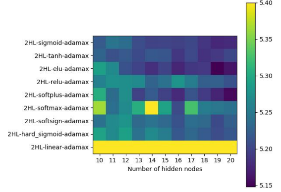
Figure 6: Output example of a systematic meta-parameters space exploration. On the x axis is represented the number of neurons per layer. On the y axis are indicated the nine tested activation functions. Here the ANN uses two hidden layers (HL) and the adamax training algorithm. Colorscale represents the performance of the ANN \sigma_{XY} as defined in the text (lower is better).
