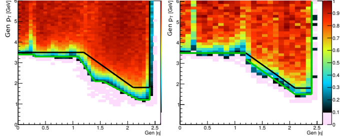
Figure 2: (p_T, |\eta|) maps of the efficiencies of reconstruction + hybrid-soft without Global requirement (left), and of reconstruction + selection + trigger (right), in PbPb. The green line is the chosen acceptance cuts, compared the ones used with 2015 data in black.
