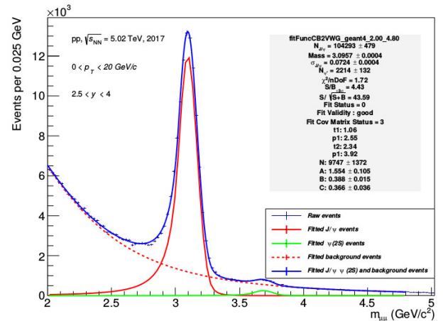
Figure 2: Inclusive J/\psi signal extraction for 0 < p_T < 20 GeV/c at forward rapidity in pp collisions.
