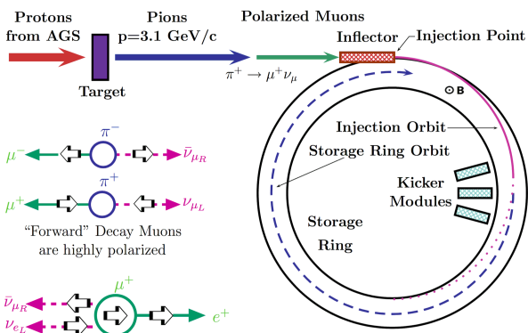
Figure 1: Sketch of BNL E821 experiment
