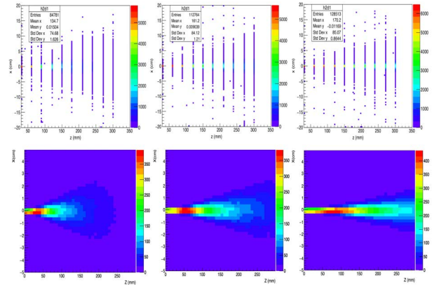
Figure 3: Horizontal beam profile along the longitudinal direction (top) and energy deposition on the x-z plane (bottom) in the water box for 70, 140 and 300 MeV Grid mini-beam respectively.
