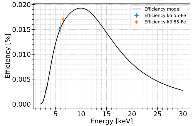
Figure 6: Detection efficiency curve of the X-PIPS TM detector SDD, at a distance of 10.3 cm from the radioactive source
