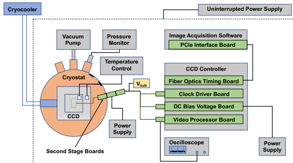
Figure 7: Apparatus for a CCD test chamber.
