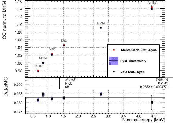
Figure 4: Non-linearity of the liquid scintillator response as resulting from the new analysis strategy. Calibration coefficient are normalized to ^{54}\text{Mn} .
