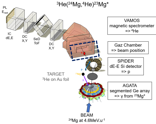
Figure 4: Layout of the GANIL experiment, for the measurement of the reaction {}^3\text{He}({}^{24}\text{Mg}, \alpha){}^{23}\text{Mg}^*(p){}^{22}\text{Na} .
