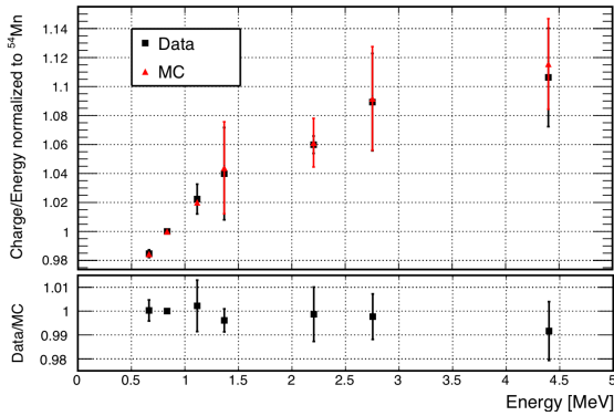
Figure 2: Non-linearity of the liquid scintillator response of the target in 2017[4]. Data and MC points are normalized to the ^{54}\text{Mn} . Data-MC ratio is normalized to the ^{54}\text{Mn} ratio.
