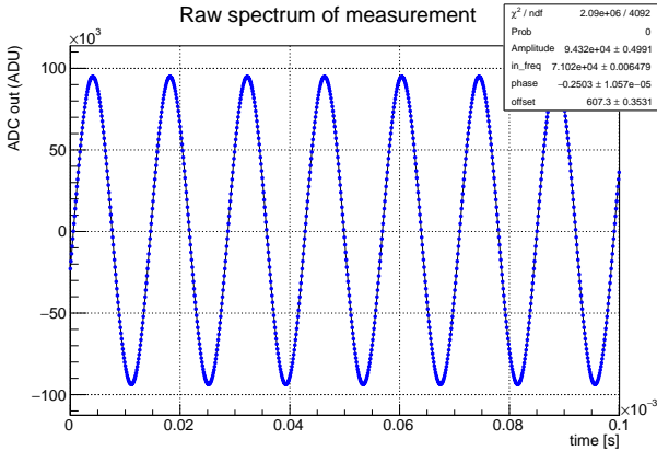
Figure 6: ADC output for sinusoidal input signal - zoomed time axis
