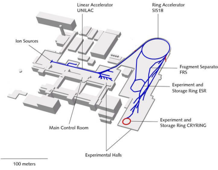
Figure 1: Schematic layout of the GSI accelerator complex used during the experiment
