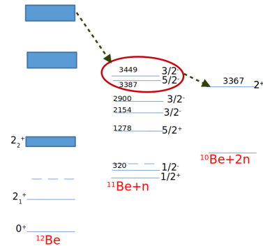
Figure 6: Higher excited resonances can decay trough states in ^{11}\text{Be} that are close to the first excited state of ^{10}\text{Be} .
