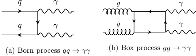
Figure 2: Examples of Feynman diagrams at the lowest order for diphoton production
