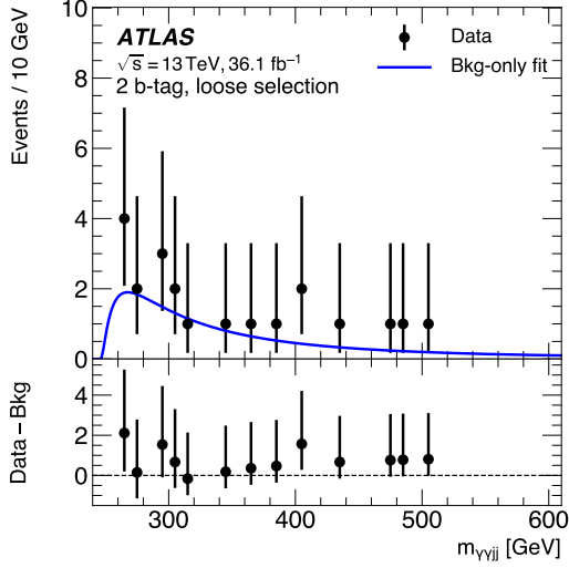
Figure 6: Data (black points) are compared with the background-only fit (blue solid line) of m_{\gamma\gamma jj} . The lower panel shows the residuals between the data and the best-fit background. [11]
