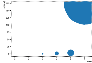
Figure 3: Masses of the six known quarks
