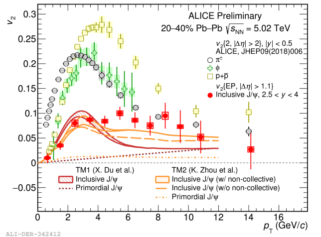
Figure 2: Inclusive J/\psi v_2 as function of transverse momentum p_T and comparison to those of light flavor charged particles (pions, protons, \phi meson) for non-central Pb–Pb collisions corresponding to 20–40% centrality class.
