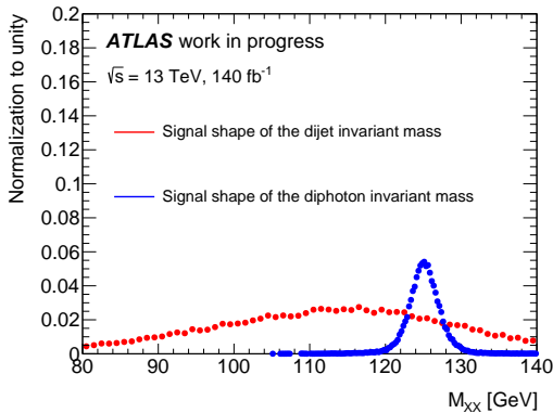
Figure 3: Invariant mass, normalized to unity, of the diphoton invariant mass in blue and of the di-jet invariant mass in red coming from a HH \rightarrow \gamma\gamma b\bar{b} decay.
