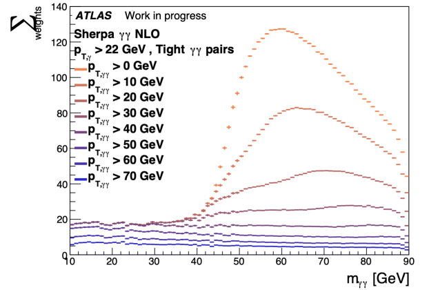
Figure 5: MonteCarlo invariant diphoton mass distributions for different transverse energy cuts. p_{T,\gamma\gamma} is the transverse momentum of the diphoton system with respect to the beam axis. The plot shows how the distribution without selection flattens when applying a boosted selection ( around p_{T,\gamma\gamma} > 50 GeV).
