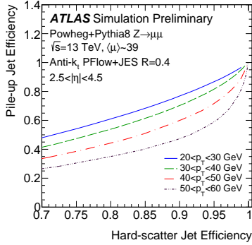
Figure 2: Efficiency for pile-up jets in simulated Z +jets events as a function of the efficiency for hard-scatter jets for different jet p_T ranges. For a standard value of hard-scatter jet efficiency the pile-up jet efficiency is improving with p_T since pile-up effects are less dominant in higher p_T bins.
