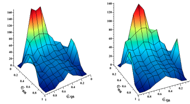
Figure 9: (Right) simulated Dalitz plot with r_{nn}^{\text{rms}} = 2.6 fm. (Left) experimental Dalitz plot.
