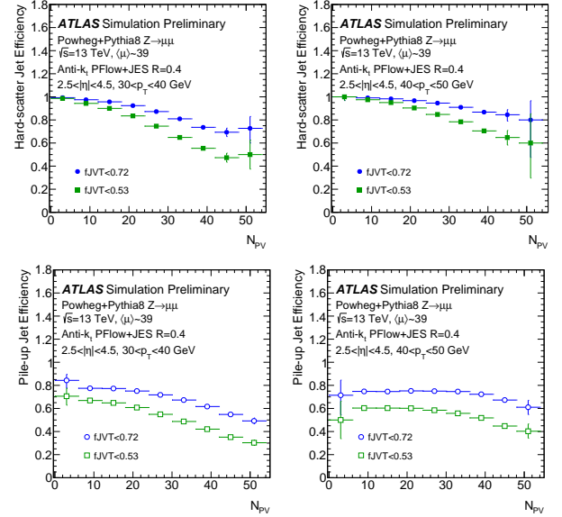
Figure 4: Efficiency in simulated Z +jets events as a function of N_{PV} for hard-scatter forward jets with 30 \text{ GeV}/c < p_T < 40 \text{ GeV}/c (top left), 40 \text{ GeV}/c < p_T < 50 \text{ GeV}/c (top right), and for pile-up forward jets with 30 \text{ GeV}/c < p_T < 40 \text{ GeV}/c (bottom left), and 40 \text{ GeV}/c < p_T < 50 \text{ GeV}/c (bottom right).
