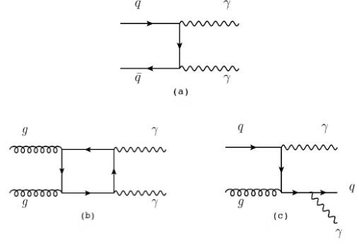
Figure 4: Example of Feynman diagram for the continuum di-photon background
