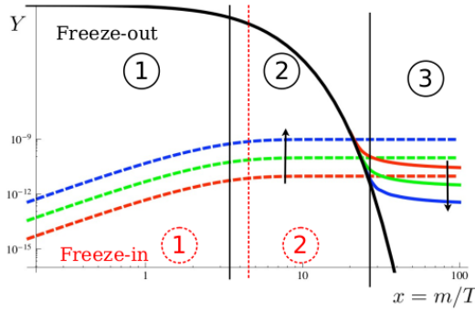
Figure 2: Evolution of the dark matter abundance as a function of x \equiv m_\chi/T for freeze-out (solid lines) and freeze-in (dashed lines). The numbers in circles delineate different phases in the evolution. Figure adapted from [6].
