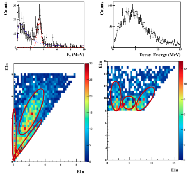
Figure 5: (Up left) ^{10}\text{Be} gamma spectrum. (up right) ^{10}\text{Be} + 2n Spectrum. (Down) bi-dimensional ( E_{fnn} , E_{fn} ) plot : (left) from 0 to 8 Mev decay energy, (right) from 8 to 15 decay energy. different forms appear on these graphs.
