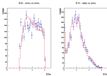
Figure 7: Fit of E_{2n} and E_{1n} spectra obtained by a project of the bi-dimensional plot: the fit is done on E_{1n} and the parameters are reported on E_{2n} .
