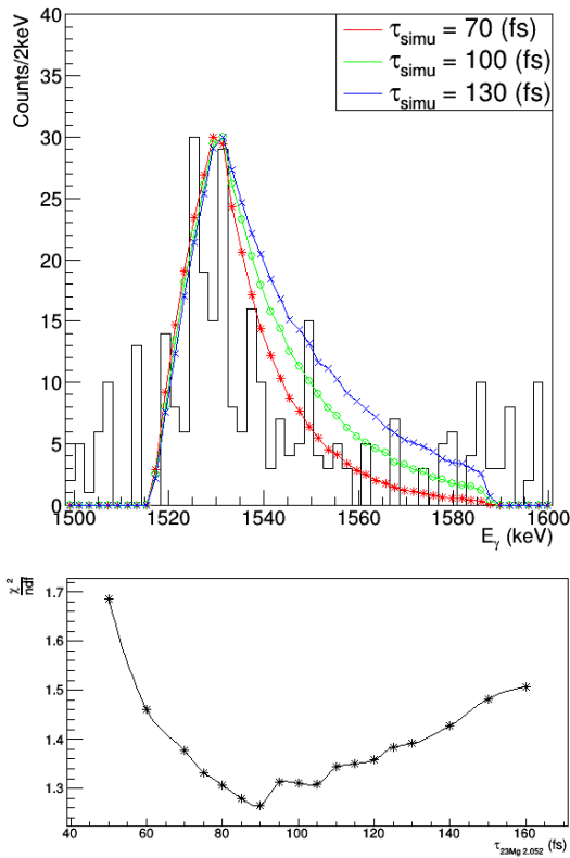
Figure 9: Analysis of the ^{23}\text{Mg} 2.052 MeV level with E_\gamma=1.601 MeV at rest. Top: experimental Doppler shifted \gamma peak with background subtraction, compared to simulated \gamma peaks with different values of lifetime (70, 100, 130) fs. Here, the selected angle is [124,133]^\circ , the \alpha gating [50.45,51.03] MeV. Bottom: \frac{\chi^2}{ndf} as a function of the simulated lifetime. The fit is made on the chosen energy window [1518,1556] keV.
