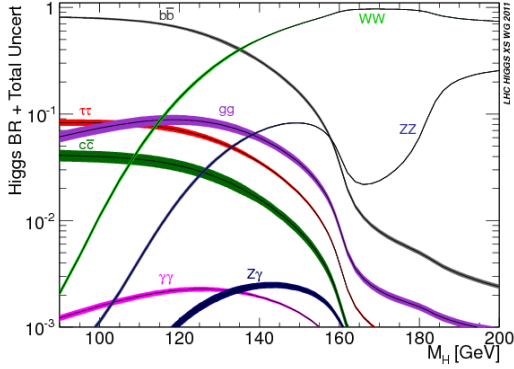
Figure 2: The SM Higgs boson branching ratios as a function of Higgs boson mass M_H . [12]
