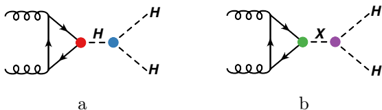
Figure 1: Feynman diagrams of a) the Higgs boson tri-linear coupling and b) a new particle and its decay in the di-Higgs boson channel
