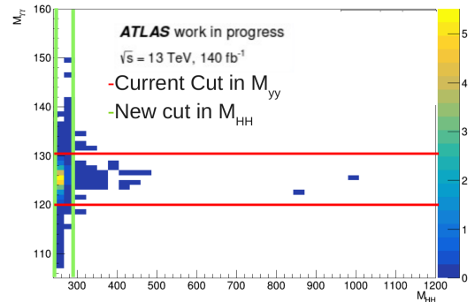
Figure 9: Distribution of the di-photon invariant mass, in the y-axis, versus the di-Higgs boson invariant mass, in the x-axis for a signal. The selection cut are represented by the green line for the new method and by the red one for the previous selection method.
