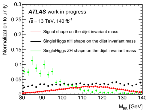
Figure 10: Number of events, normalized to unity, as a function of the di-jet invariant mass for different Single Higgs boson backgrounds and a Signal. In black for the t\bar{t}H background, in green for the ZH background and in red for the Signal
