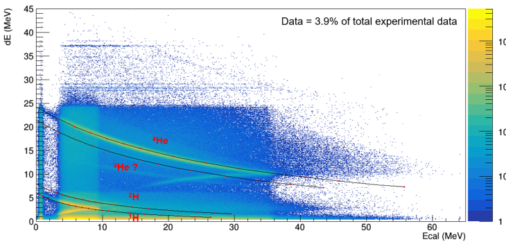
Figure 5: SPIDER dE vs E_{\text{residual}} on 3.9% of total experimental run time. Black curves are simulated energy losses of (H, He) isotopes in Si, using referenced SRIM stopping powers.
