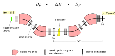
Figure 2: Sketch of the FRS. The B\rho - \Delta E - B\rho method is applied using dipoles to bend the beam ( B\rho ) as well as a degrader to have a position and Z -dependent energy loss ( \Delta E ) (figure taken from [3])
