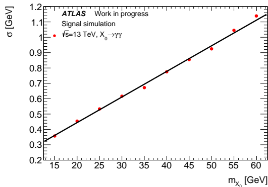
Figure 6: Width \sigma of different signal simulations as a function of the mass of a hypothetical particle X_0 . Red points show the fit results of the Double-Sided Crystal Ball and the black line the parametrized trend of the width as a function of the mass.
