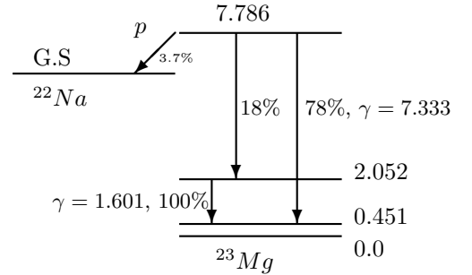
Figure 3: Decay scheme of the E_r = 0.213 MeV ( E_x = 7.786 MeV) ^{23}\text{Mg}^* level, B_p from \beta delayed proton decay of ^{23}\text{Al} [6] and B_\gamma from [5]. \gamma rays are given for the deexcitations of interest.
