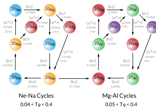
Figure 1: Nucleosynthetic cycles in ONe Novae. Production and destruction channels of ^{22}\text{Na} are shown in the upper left. Temperature range T_9 correspond to nova environments. From [2].
