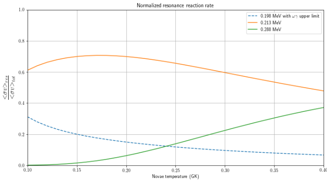
Figure 2: Normalized resonant reaction rates as a function of the temperature, using \omega\gamma measured in Ref. [3] for the three resonances (0.198, 0.213, 0.288) MeV.
