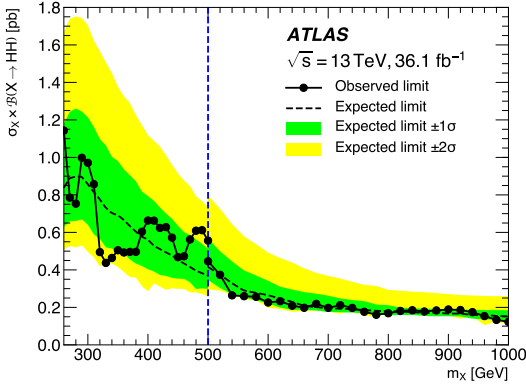
Figure 7: The expected and observed 95% CL limits on the resonant production cross-section, \sigma_X \times \mathcal{B}(X \rightarrow HH) as a function of m_X . [11]
