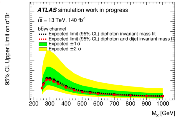
Figure 12: Cross section upper limit as a function of the invariant mass of the possible new particle. The limit is computed using the new 2D fit method in red and using the fit on the di-photon invariant mass in black
