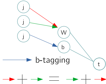
Figure 7: Schematic of the two approaches to reduce the number of possible jet permutations.
