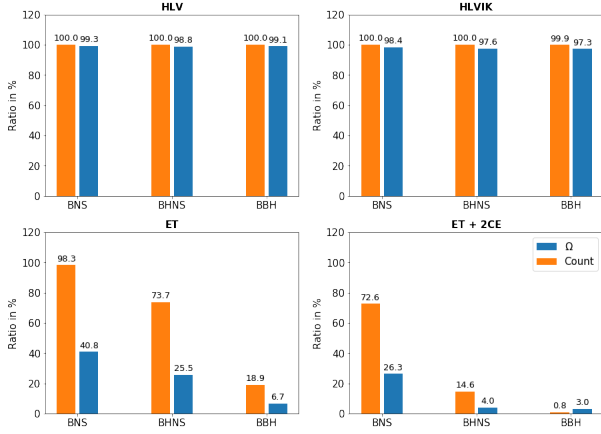
Figure 3: Ratio for residual backgrounds for the total population I/II and III. The blue bars exhibits the ratio in energy density, while the orange ones shows the ratio by counting sources in the residual background.
