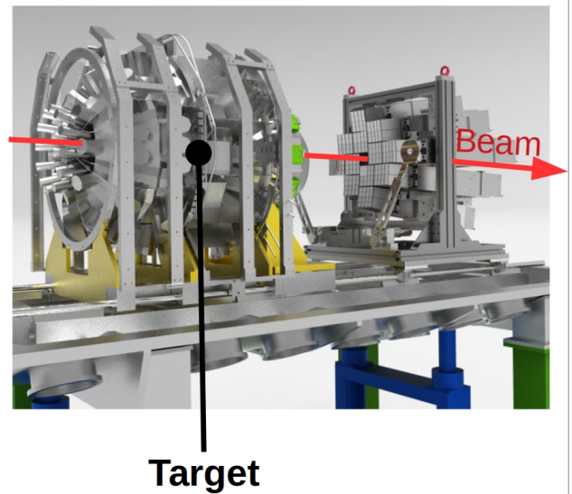
Figure 1: Left side INDRA, right side FAZIA
