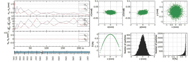
Figure 10: Beam optics (left) and phase space (right) of FCC-ee 4.46 GeV linac
