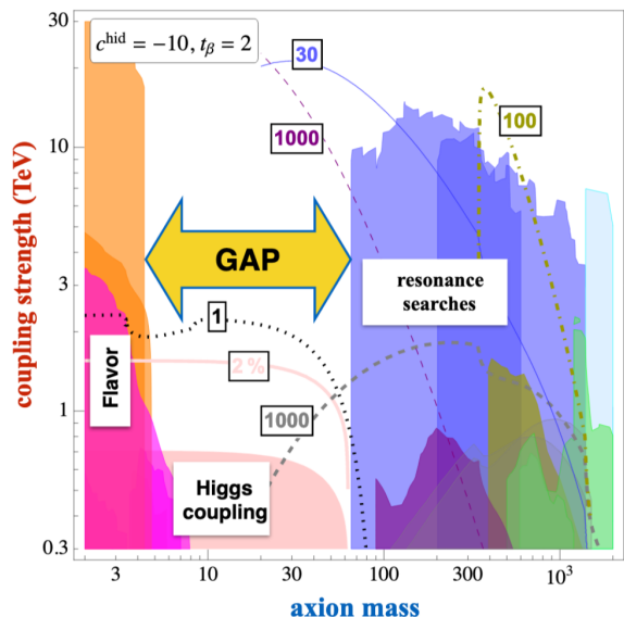
Figure 1: Existing searches and constraints in the parameter space for resonance searches. The plot shows the coupling strength as a function of the mass of the ALP. The research “gap” lies between 5 GeV up to 65 GeV, the mass range of this analysis [4].
