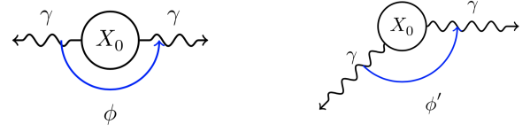
Figure 4: Transverse view of back-to-back (left) and boosted (right) decays from a hypothetical X_0 ALP to two photons of equal energy. For photons in the boosted topology the invariant mass is lower compared to the back-to-back scenario.
