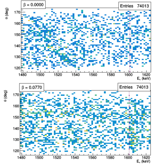
Figure 7: AGATA reconstructed angle \theta_\gamma versus Doppler corrected energy E_\gamma . From top to bottom, Doppler correction is applied at the two \beta values 0.0 and 0.077. Dashed purple line at 1601 keV marks the expected \gamma -line from the ^{23}\text{Mg} 2.052 MeV level. Here, the \alpha energy gate is [50.45,51.03] MeV.
