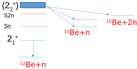
Figure 4: An unbound resonance above 2n emission threshold is observed and its decay modes are analysed
