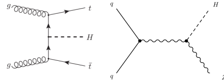
Figure 5: Feynman diagram for the t\bar{t}H Higgs boson background in the left part and for the ZH Higgs boson background in the right part
