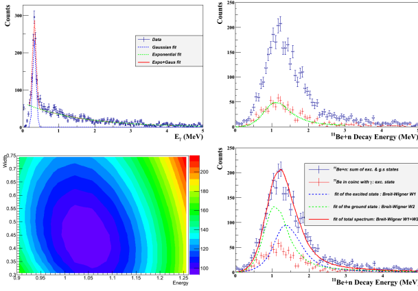
Figure 3: (Up left): gamma spectrum in coincidence with ^{11}\text{Be} + n . (Up right): total ^{11}\text{Be} + n spectrum in blue (excited + ground states) and in red is the spectrum of ^{11}\text{Be} + n in coincidence with gamma. (Down left): \chi^2 graph for the fit of ^{11}\text{Be} + n spectrum. (Down right) Total fit of the ^{11}\text{Be} + n spectrum giving the central energy of the resonance at 1360 keV above S(n) level and the proportion of excited/ground state (60/40).
