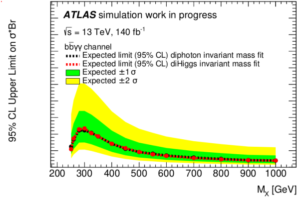
Figure 11: Cross section upper limit as a function of the invariant mass of the possible new particle. The limit is computed using the old method in red and using the fit on the di-photon invariant mass in black
