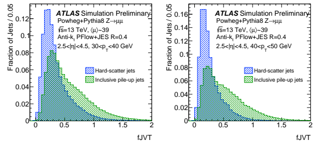
Figure 1: fJVT distributions for hard-scatter (blue) and pile-up (green) forward jets with 30 < p_T^{\text{jet}} < 40 \text{ GeV}/c (left) and 40 < p_T^{\text{jet}} < 50 \text{ GeV}/c (right).
