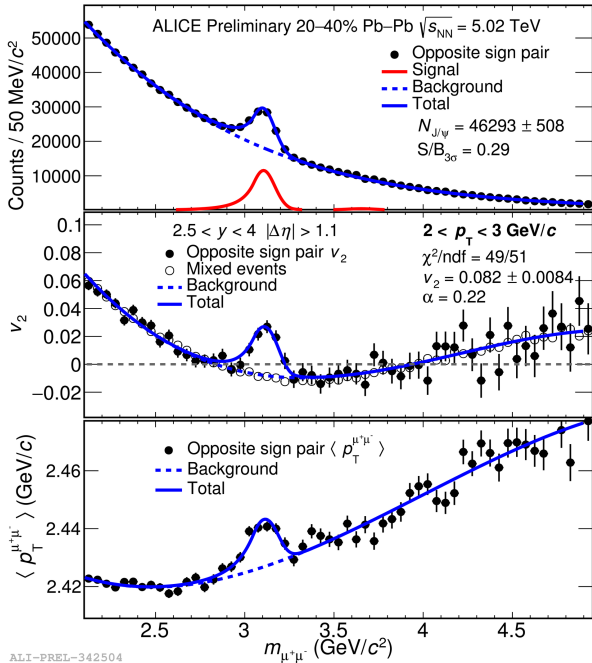
Figure 1: (Top) J/\psi signal extraction using the dimuon invariant mass spectrum. (Middle) Total dimuon v_2 as function of m_{\mu\mu} and the corresponding fitting functions as the formula (5), each black circle corresponds to the average v_2 value of all dimuons in one bin of m_{\mu\mu} . (Lower) Extraction of the \langle p_T \rangle^{J/\psi} corresponding to the fit on total dimuon \langle p_T \rangle .
