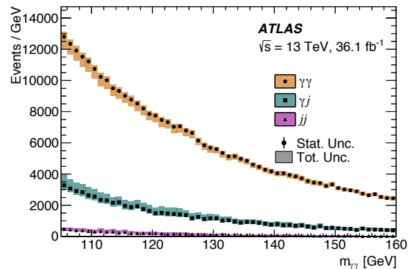
Figure 7: Event yields as a function of the invariant mass of the diphoton pair for the three non-resonant background contributions in the range between 105 and 160 GeV [5].
