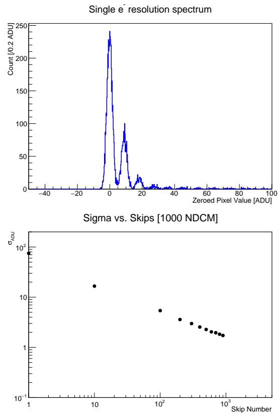
Figure 8: DAMIC-M CCD single electron resolution.
