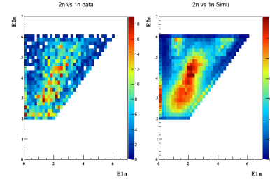
Figure 8: (Right) simulated bi-dimensional plot with two resonances: 4.6 and 6.5 MeV. (Left) experimental bi-dimensional plot
