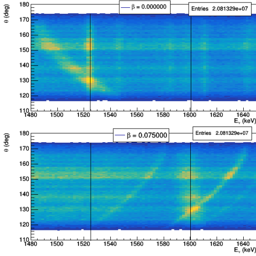
Figure 6: AGATA reconstructed angle \theta_\gamma versus Doppler corrected energy E_\gamma . From top to bottom, Doppler correction is applied at two \beta values: 0.0 and 0.075. Black lines at 1528 and 1601 keV mark the expected \gamma decays of respectively, the ^{22}\text{Na} 1.528 MeV level and ^{23}\text{Mg} 2.052 MeV level.
