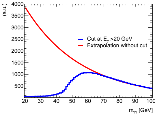
Figure 3: Invariant mass distribution for diphoton pairs with each photon transverse energy E_{T,\gamma} > 20 GeV compared to an extrapolated distribution of diphoton pairs without this selection. The shape of the distribution changes significantly around twice the value of the p_T selection.
