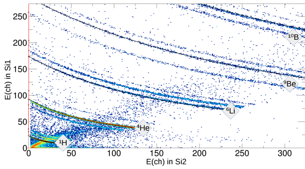
Figure 10: \Delta E - E in Si1-Si2
