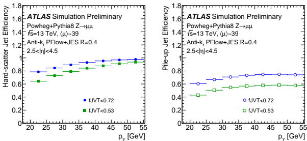
Figure 3: Hard-scatter (left) and pile-up (right) jet efficiency as a function of forward jet p_T for simulated Z +jets events.
