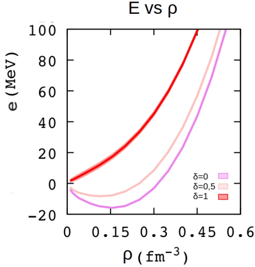
Figure 2: Figure from [2]. For \delta=1 pure neutron nuclear matter, for \delta=0 symmetric nuclear matter, for \delta=0.5 asymmetric nuclear matter.
