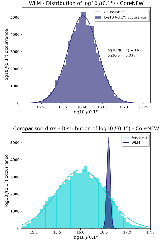
Figure 1: Histograms and fits (solid lines) of the results of the MCMC on the coreNFW profile parameters [5] for a ROI (Region of Interest) of 0.1^\circ . Top: Distribution of the J factor for WLM. The nominal J factor and its uncertainties are the mean and \sigma values respectively of the fit. Bottom: Comparison of the J factor of WLM and Aquarius and their uncertainties on J . This comparison shows WLM has a larger J factor with smaller uncertainties than Aquarius.
