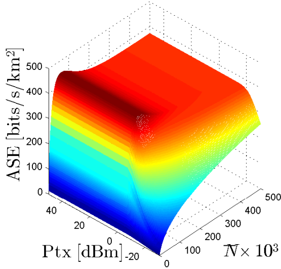
Fig. 8. The summed area spectral efficiency as a function of both the average number of EDs \bar{N} and the transmit power P_{\text{tx}} under random SF allocation scheme.
