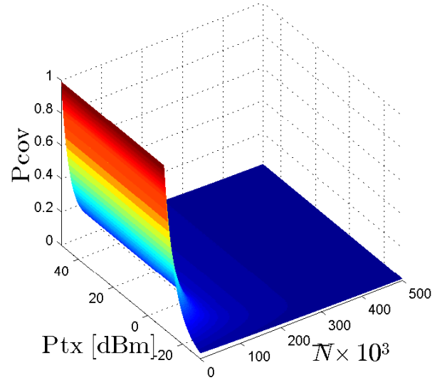
Fig. 7. The coverage probability as a function of both the average number of EDs \bar{N} and the transmit power P_{tx} under fair SF allocation scheme for SF k = 8 .
