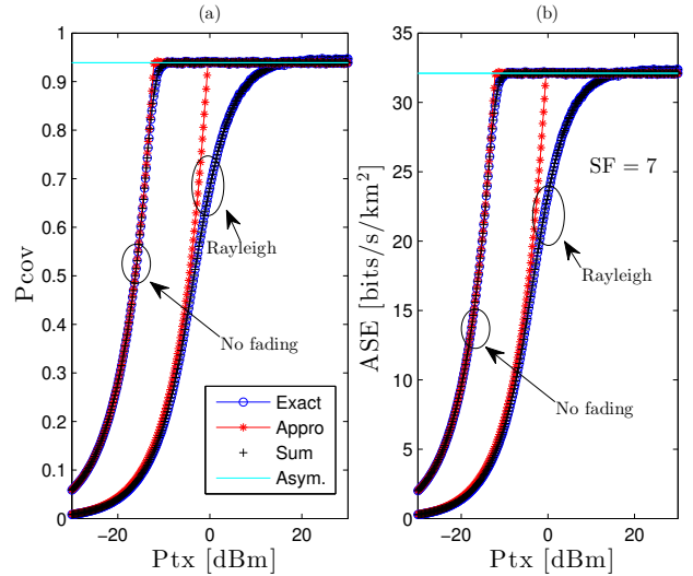
Fig. 1. Coverage probability (a) and area spectral efficiency (b) versus the transmit power under random SF allocation scheme. The marked solid lines show the exact, and approximate analytical framework, while the plain solid line shows the asymptotic behavior when P_{\text{tx}} \rightarrow \infty for both the Pcov and ASE as computed by equations (7), (8) and (9). The markers show the respective Monte Carlo simulations.
