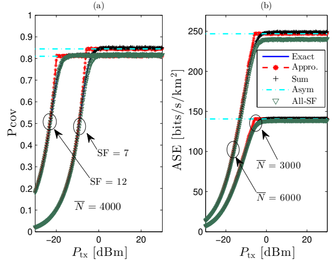
Fig. 3. Coverage probability (a) and area spectral efficiency (b), versus P_{tx} under a fair-collision SF allocation scheme. The solid lines correspond to the exact framework of (7), and (9); the dashed lines show the approximate framework of (8) and (9) and the dotted dashed lines show the asymptotic behavior as P_{tx} \rightarrow \infty . The plus sign markers show the Monte Carlo simulations accounting only for the aggregate interference intra-SF interferer, while the downward-pointing triangles show the simulations considering the aggregate interference (of all inter-SF and intra-SF interferers).
