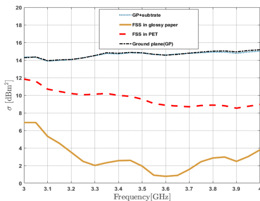
Figure 14: RCS measurement results of the FSS structure
