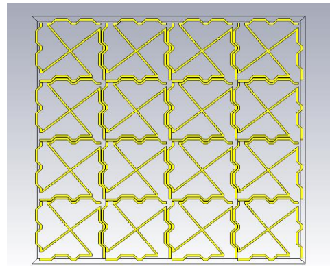
Figure 6: Freestanding FSS structure with interdigitating of adjacent metallic bands
