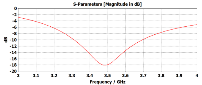
Figure 11: Simulation of the reflection coefficient of the compact FSS structure of Fig. 10
