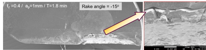
(c) a_p = 1mm , t = 1mm , \gamma_n = -15^\circ
