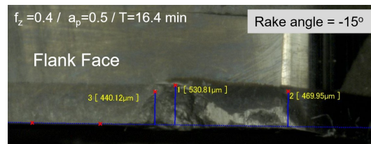
(a) a_p = 0.5mm , t = 16mm , \gamma_n = -15^\circ
