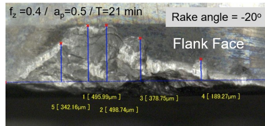
(b) a_p = 0.5mm , t = 21mm , \gamma_n = -20^\circ
