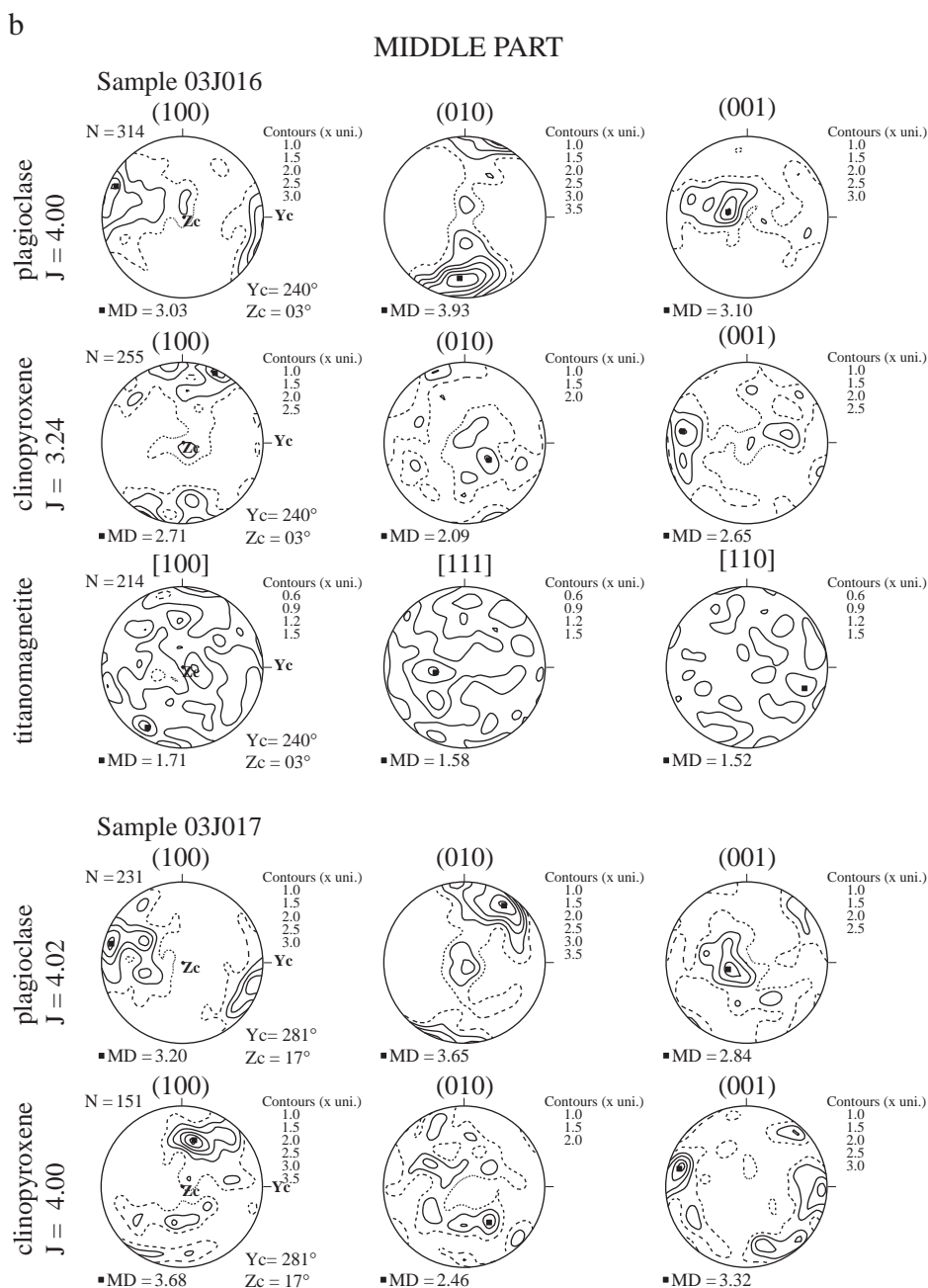
Fig. 6. Lattice Preferred Orientation of plagioclase, clinopyroxene and titanomagnetite of samples from the lower and the upper part (a), and the middle part (b) of the flow. Equal area projection in the lower hemisphere and in the specimen coordinate system with Yc the specimen azimuth and Zc the dip of the drilled core ( Zc=90^\circ for a vertical core). Contours are in Multiples of Uniform Distribution (M.U.D). J is the texture index and N the number of measurements.
