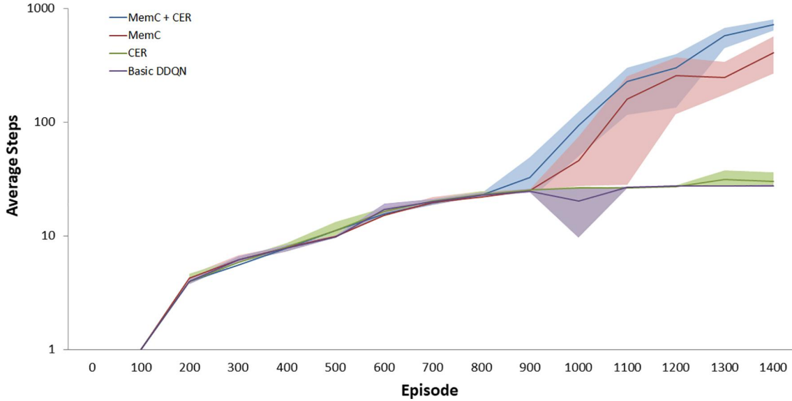
FIGURE 5 Comparison of the learning performance of the basic double deep Q-network (DDQN)-energy management system (EMS) and the three proposed variants of DDQN-EMS a with combined experience replay ( CER ), with the memory counter ( MemC ), with both ( MemC + CER )
