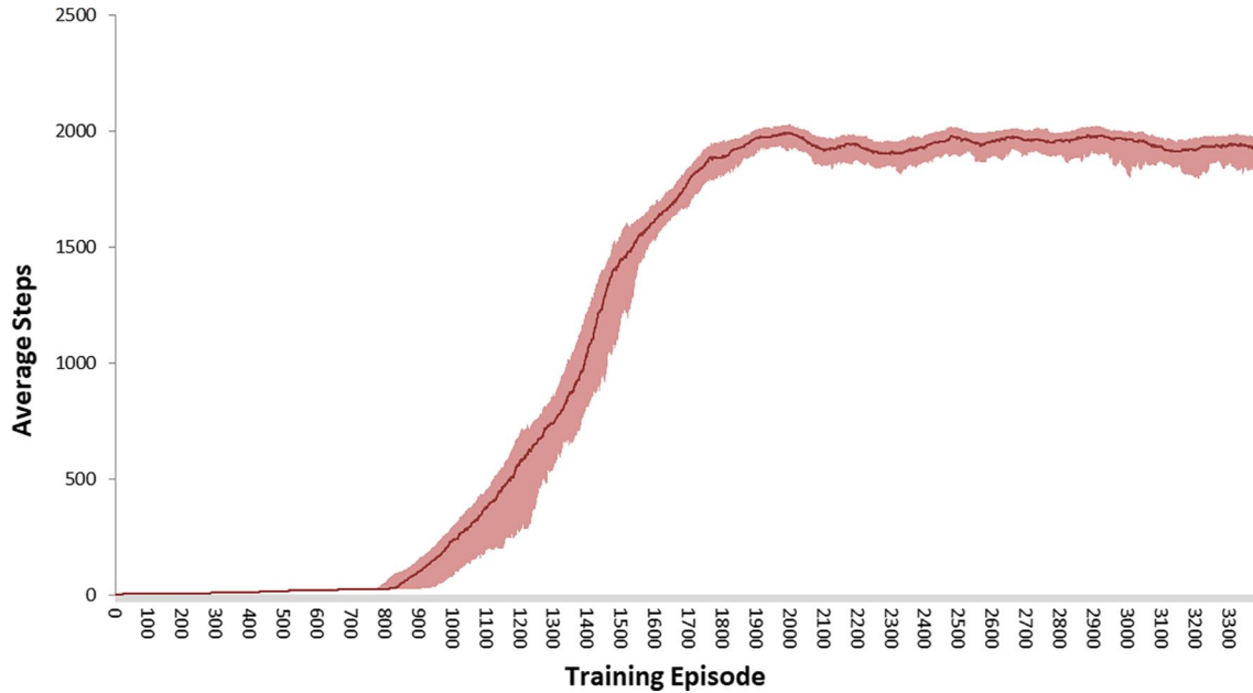
FIGURE 7 Learning curve of the DDQN-EMS a algorithm
