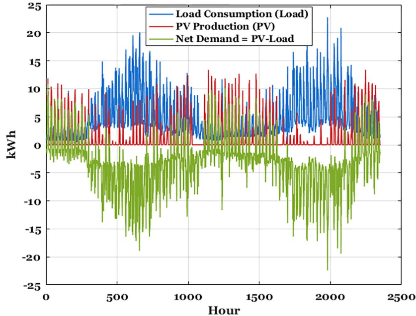
FIGURE 4 The dataset of load consumption, PV power production and net demand
