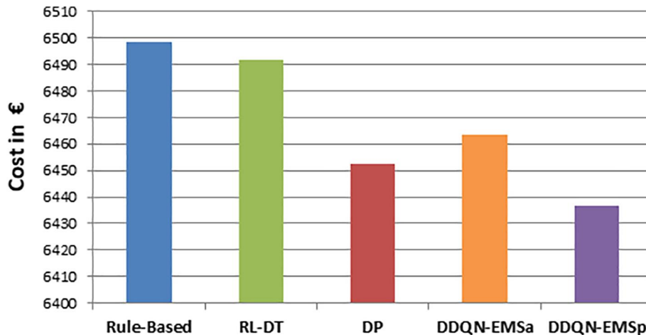
FIGURE 8 Performance of the competing algorithms: see text for details
