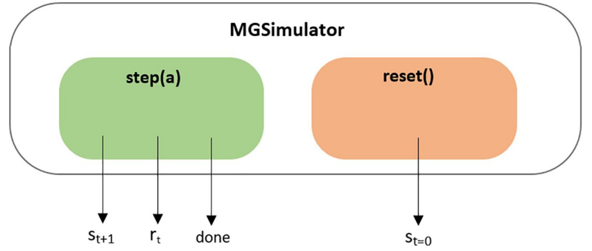
FIGURE 2 The MGSimulator architecture. The two main function: step in green and reset in orange are illustrated. Arrows return the results of the functions
