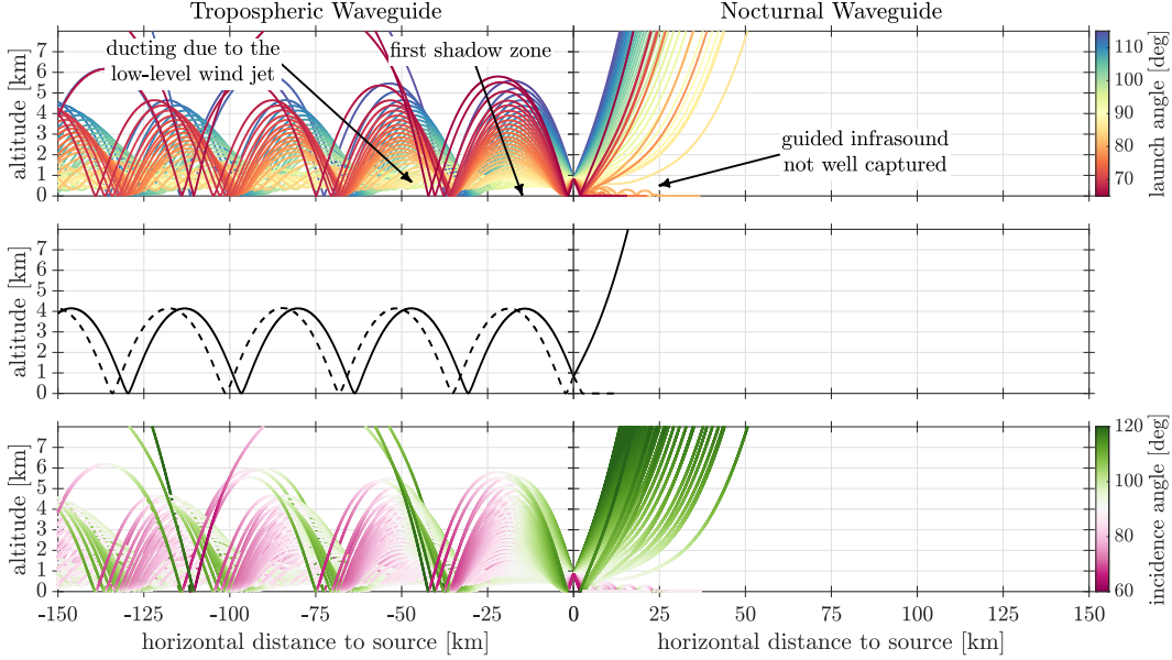
Figure 6. Acoustic rays propagation in the tropospheric and nocturnal waveguides, on the left and right panels respectively. Top: rays color-coded with launch angle. Middle: ray trajectories for a couple of launch angles ( 70^\circ as dashed line, and 110^\circ as plain line). Bottom: rays color-coded with incidence angle with respect to the direction of propagation. Rays are traced using the reference background model (sol 0, 20h LMST, landing site location, plotted in Supplementary Figure S1).
