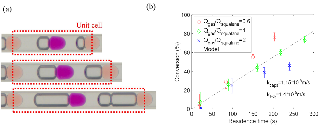
Fig.16: (a) Photos of the unit cell for the experiments on the gas influence, from top to bottom Q_{gas}/Q_{squalane}=0.6 , Q_{gas}/Q_{squalane}=1 , Q_{gas}/Q_{squalane}=2 , (b) Experimental conversion and results from the simulation.
