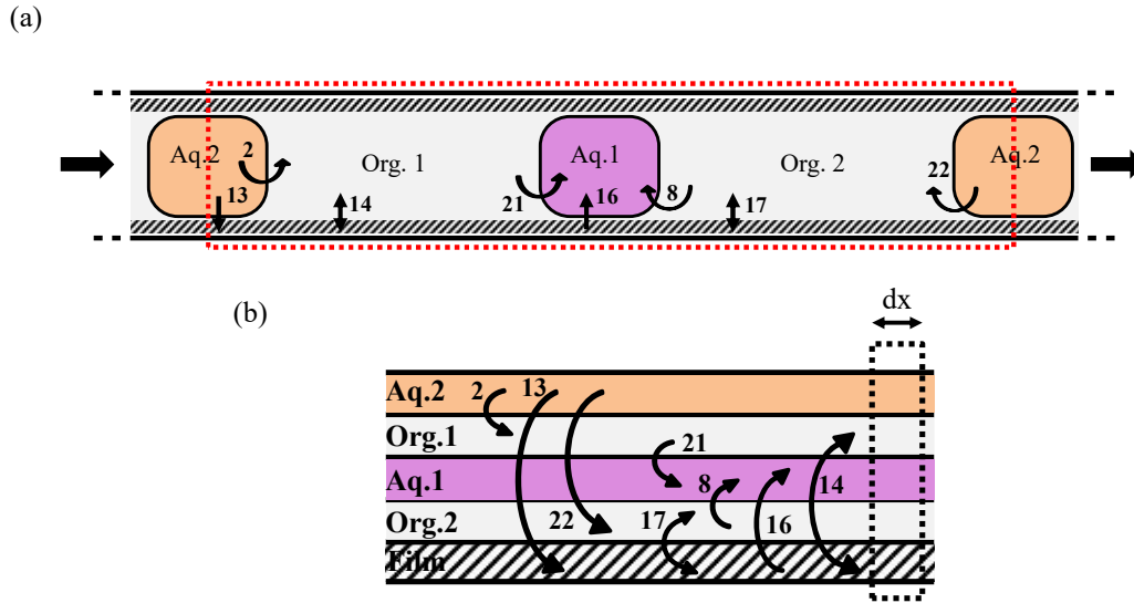
Fig.13: (a) Schematic illustration of the unit cell without gas with the transport processes of interest for the model, (b) Schematic illustration for the plug flow steady state modelling approach.
