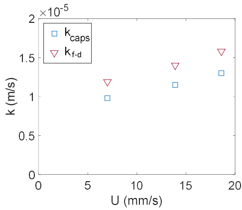
Fig.15: Influence of superficial velocity on the mass transfer coefficient k_{caps} and k_{f-d}
