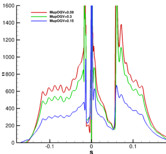
Figure 9 : Variation of htc with upstream Mach number ( M_{up} OGV) for a conjugate model ( k-l model)
