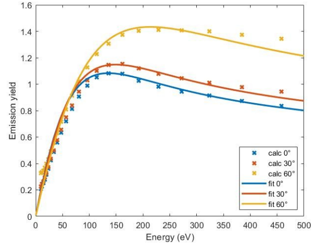
Fig. 6. Fitted electron emission yield for simulated data at 0^\circ . The emission yield at higher angles has been deduced from the fit at 0^\circ with the formula given in equation (6).
