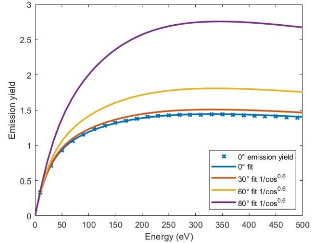
Fig.7. Fitted electron yield curve with different angular dependencies to fit the electron yield curves at higher angles of incidence. For the model a value of a = 0.6 was chosen, from the results of the calculated yield curves. The backscattered electrons have been removed according to equation (4).
