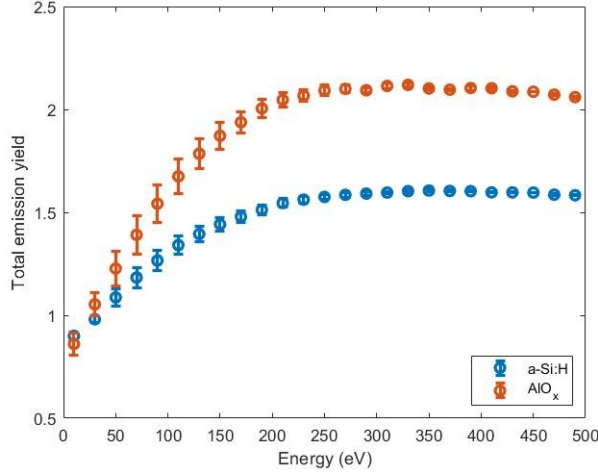
Fig. 4. Experimental electron emission yield, measured at 0^\circ incidence at the ONERA Space Lab.
