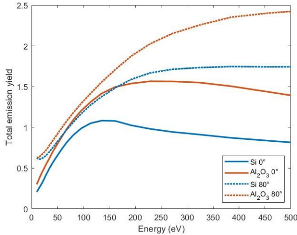
Fig. 5. Simulated electron emission yield of Si and \text{Al}_2\text{O}_3 at angles of incidence of 0^\circ and 80^\circ .
