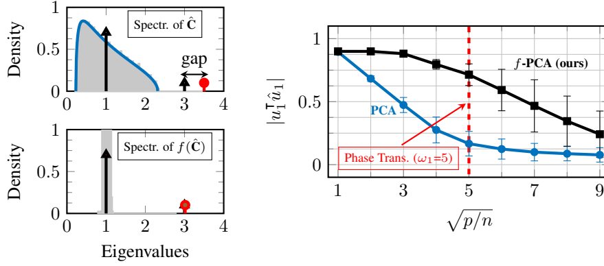
Figure 1: (Left) Spectrum of \hat{C} (up) and f(\hat{C}) (bottom) for p = 2048 and n = 7500 . Limiting Marčenko-Pastur density (Marčenko & Pastur, 1967) in blue versus spectrum of \Sigma_p in black, with \omega_1 = 2 ; estimated largest eigenvalue in red. (Right) Alignment between estimated PC and GT (the “Three Peak” example of (Johnstone & Lu, 2009) in the “Symmlet 8” wavelet basis), in terms of \sqrt{p/n} . We considered \omega_1 = 5 and thus the phase transition for standard PCA occurs at \sqrt{p/n} = 5 , thereby suggesting another phase transition for f -PCA. Curves obtained from 500 realizations of X .
