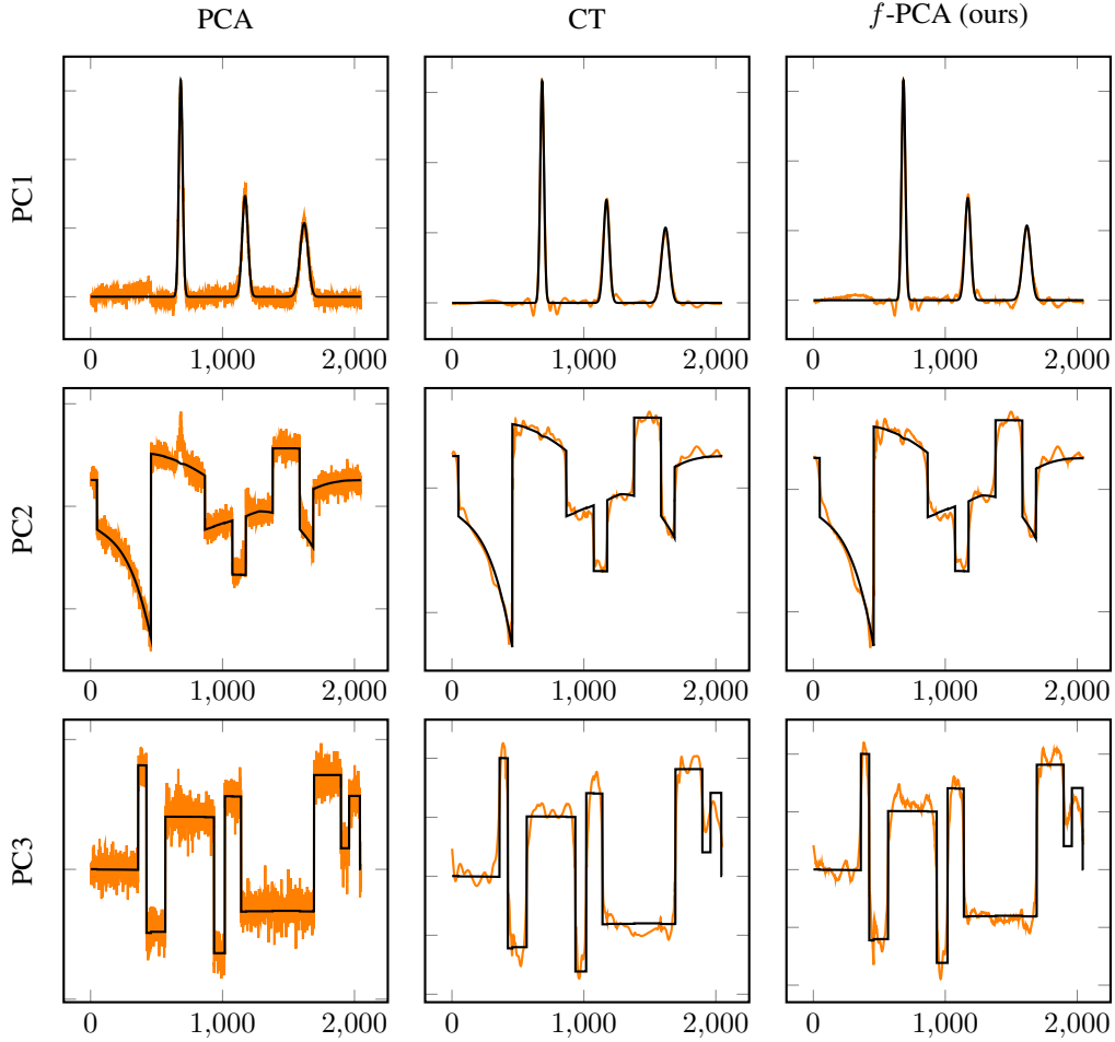
Figure 4: Multiple principal components ( k = 3 ) recovery (in orange) with standard PCA ( left ), the CT method ( middle ) and our method ( right ) where the PCs are considered to be the “Three Peak”, “Piece Poly” and “Step New” signals of (Johnstone & Lu, 2009), in the “Symmlet 8” wavelet basis. We use p = 2048 , n = 1024 and the spikes strengths are set respectively as \omega_1 = 100 , \omega_2 = 75 and \omega_3 = 50 . In particular, we note the similarity between the results obtained by our method and CT.
