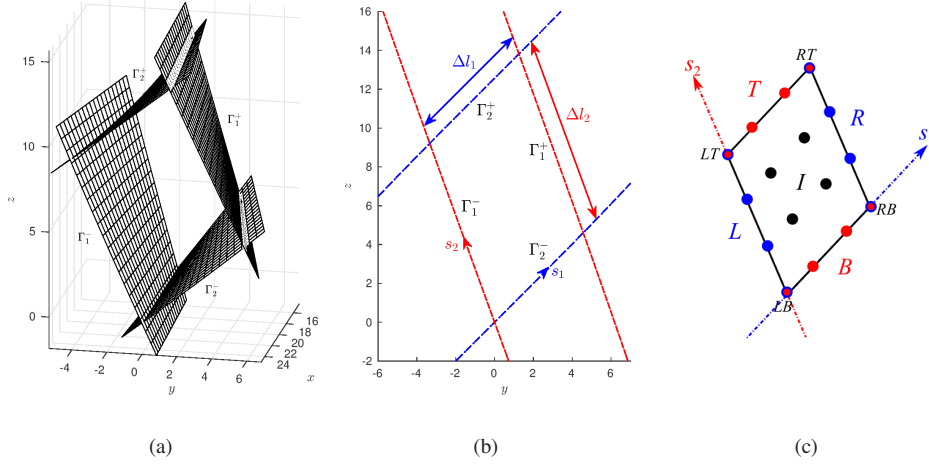
Figure 4: Cutting surfaces of the unit cell, \Gamma_1^-(s_1 = 0) , \Gamma_1^+(s_1 = \Delta l_1) , \Gamma_2^-(s_2 = 0) , \Gamma_2^+(s_2 = \Delta l_2) . (a) Three-dimensional view, (b) two-dimensional view, (c) classification of the boundaries of the unit cell into left ( L ), right ( R ), bottom ( B ), top ( T ) boundaries excluding the four corners LB , RB , LT , RT (the remaining part of the unit cell is the internal ( I ) region, bullets represent FE nodes). In this example, the directions s_1 and s_2 are right-handed and left-handed respectively ( \phi_1\phi_2 < 0 ).
