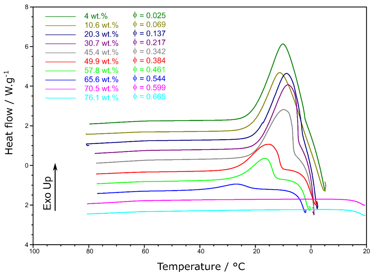
Figure S1. Cooling Differential Scanning Calorimetry scans obtained at 10\text{ }^{\circ}\text{C}.\text{min}^{-1} for alginate/water binary mixtures ranging from 4 to 76.1 wt.% in alginate.
