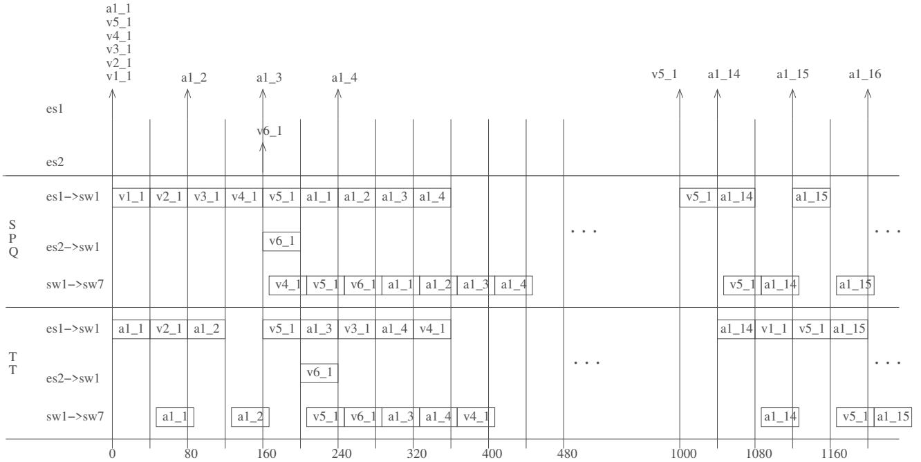
Fig. 4. Scheduling at the end system level
