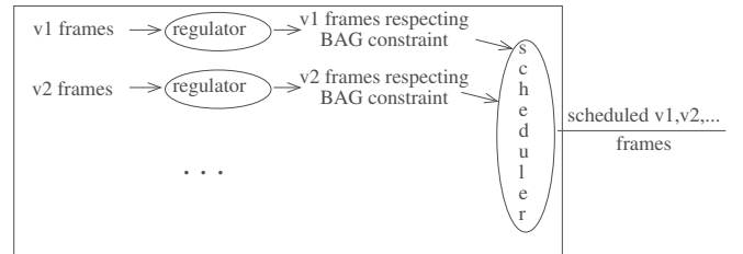
Fig. 2. End system architecture
