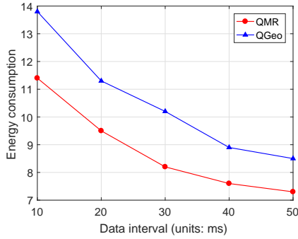
Fig. 7: Energy consumption for different data interval
