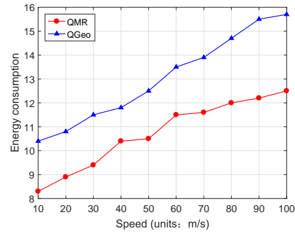
Fig. 10: Energy consumption for different moving speed
