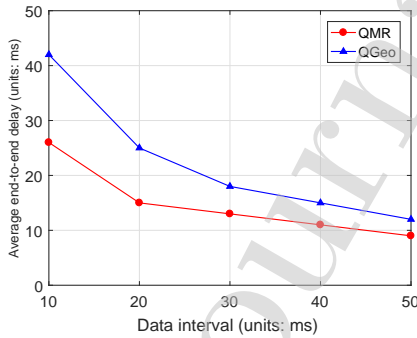
Fig. 13: Average end-to-end delay for a scenario with faulty relay nodes
