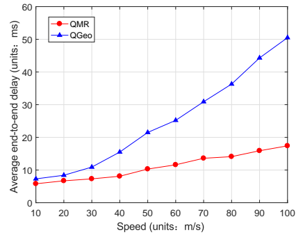
Fig. 11: Average end-to-end delay for different moving speed
