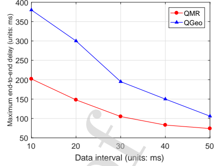
Fig. 14: Max end-to-end delay for a scenario with faulty relay nodes
