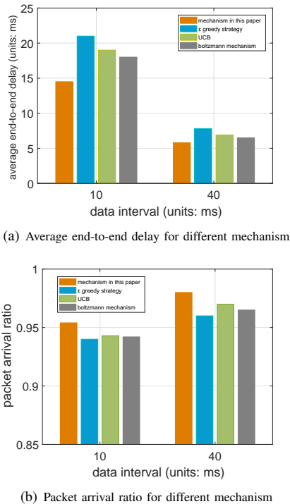
Fig. 17: Comparison of exploration and exploitation mechanism
