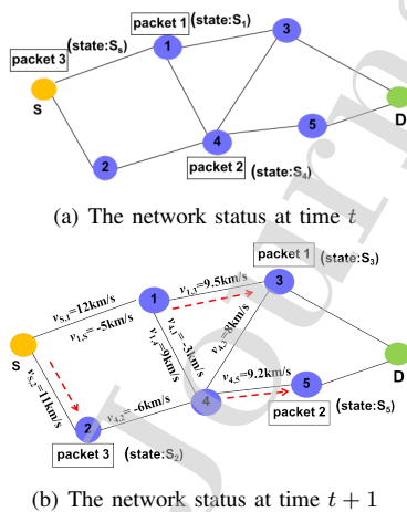
Fig. 4: The network status at time t and t + 1
