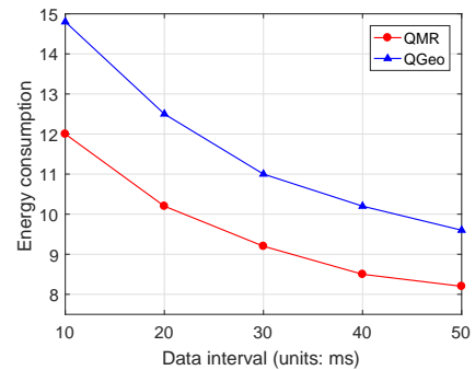
Fig. 16: Energy consumption for a scenario with faulty relay nodes
