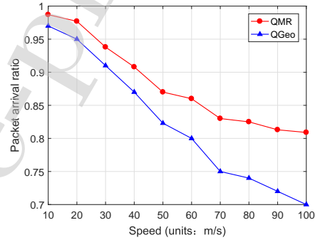
Fig. 9: Packet arrival ratio for different moving speed
