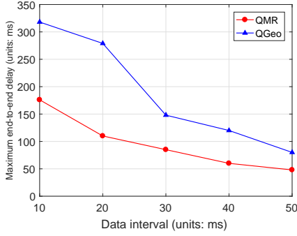
Fig. 6: Max end-to-end delay for different data interval
