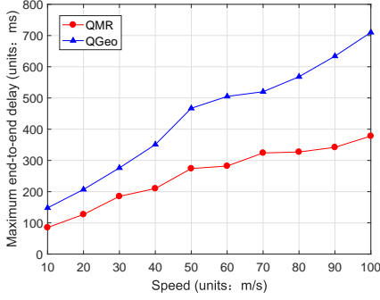
Fig. 12: Max end-to-end delay for different moving speed
