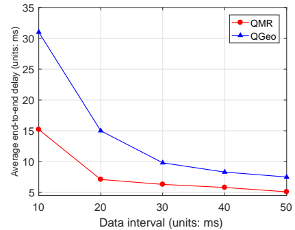
Fig. 5: Average end-to-end delay for different data interval
