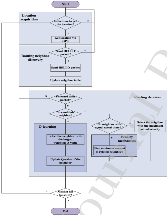
Fig. 3: Flowchart of QMR framework
