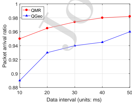
Fig. 8: Packet arrival ratio for different data interval
