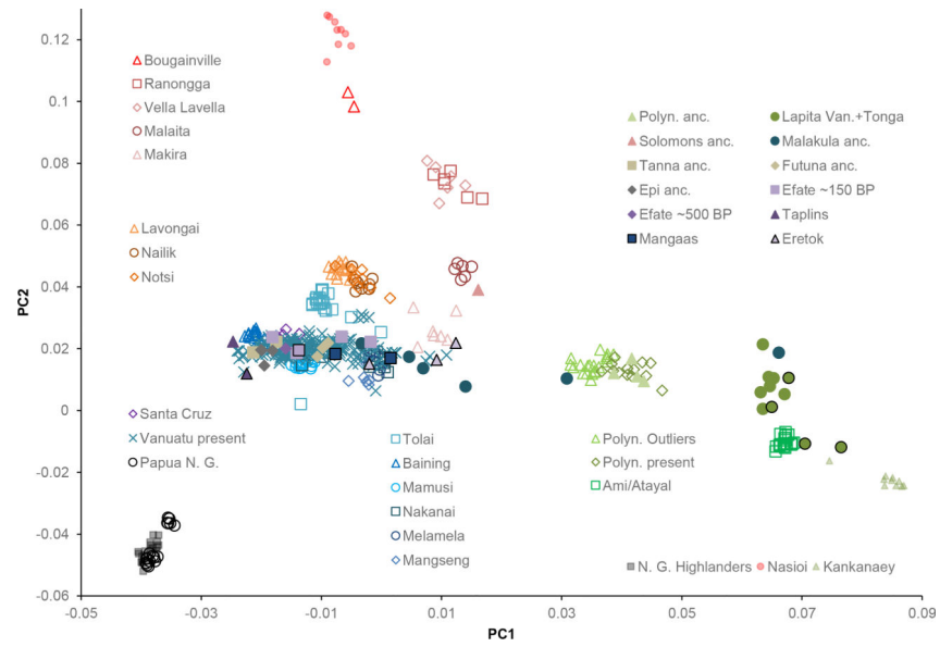
Figure 2. PCA results.
