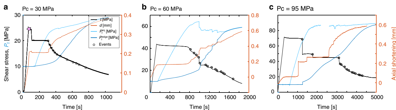
Fig. 2 Triggering of instabilities along a critically loaded crack. Evolution of the macroscopic shear stress and of the total axial shortening recorded by external gap sensors during experiments conducted at 30 (a), 60 (b) and 95 (c) MPa confining pressure. The data presented in figure a include also the loading up to the peak strength of the fault, denoted by the pink star. Before each injection, the shear stress was first placed at 90% of the peak strength of the fault. Then, fluid was injected at a constant volume rate into the injection borehole (Supplementary Fig. 1a), up to the release of the energy stored in the system. Black, red, cyan and blue solid lines correspond to the evolution of the shear stress, the fault slip, the fluid pressure in the injection borehole and the fluid pressure in the measurement borehole, respectively. Black circles correspond to each slip instability treated in this study. The missing data in panel c are related to experimental maintenance of the fluid pressure system. The fluid pressure during this period is constant along the experimental fault.
