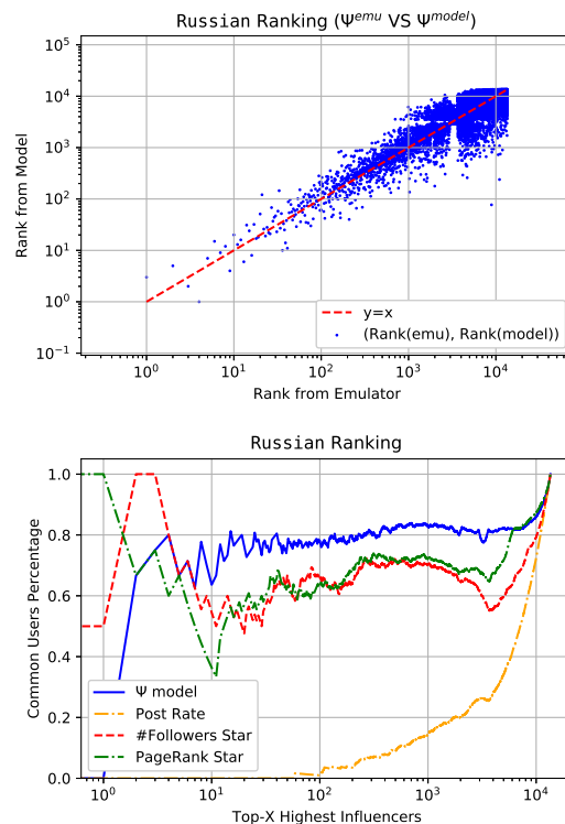
Fig. 6. User ranking comparison for Russian. (a) top: Scatter plot between \text{Rank}(\Psi^{\text{model}}) and \text{Rank}(\Psi^{\text{emu}}) – points on the left rank higher (1st, 2nd, etc.), (b) bottom: Common users proportion with reference to \text{Rank}(\Psi^{\text{emu}}) .
