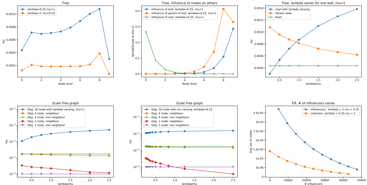
Fig. 4. Top: Binary Tree. (a. left) \Psi -score per tree level, (b. centre) \mathbf{q} -influence vector over a branch, (c. right) Change of \Psi -scores by increase of \lambda_{leaf} ; Bottom: Change of \Psi -scores in a scale-free graph when (d. left) \lambda_{deg=20} increases, (e. centre) \mu_{deg=20} decreases, (f. right) E-R graph tragedy of commons.
