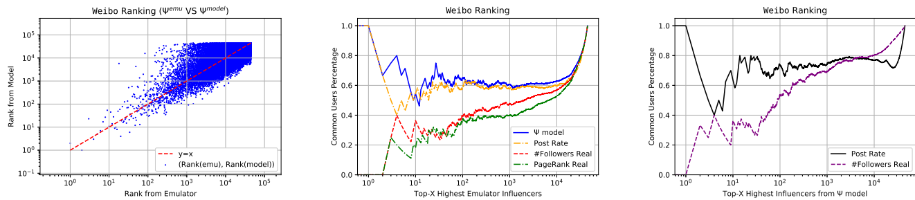
Fig. 7. User ranking comparison for Weibo. (a) left: Scatter plot between \text{Rank}(\Psi^{\text{model}}) and \text{Rank}(\Psi^{\text{emu}}) – points on the left rank higher (1st, 2nd, etc.), (b) centre: Common users proportion with reference to \text{Rank}(\Psi^{\text{emu}}) , (c) right: Common users proportion with reference to \text{Rank}(\Psi^{\text{model}}) .
