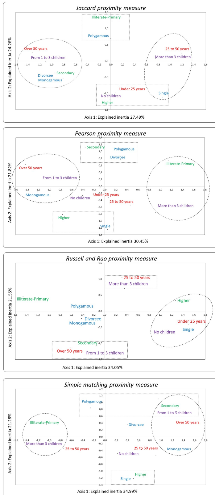
Fig. 5. Jaccard (Class 1), Pearson (Class 2), Russel & Rao (Class 3) and Simple Matching (Class 4) proximity measures.
