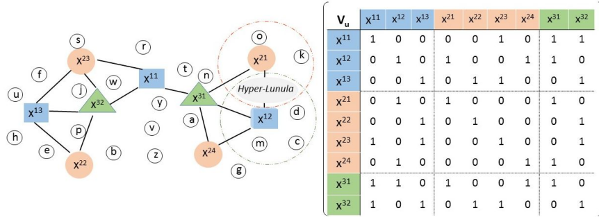
Fig. 1. RNG example with nine groups-modalities and associated adjacency matrix
