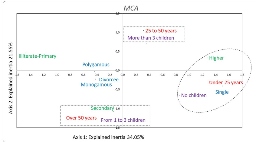
Fig. 4. MCA - Graphical representation
