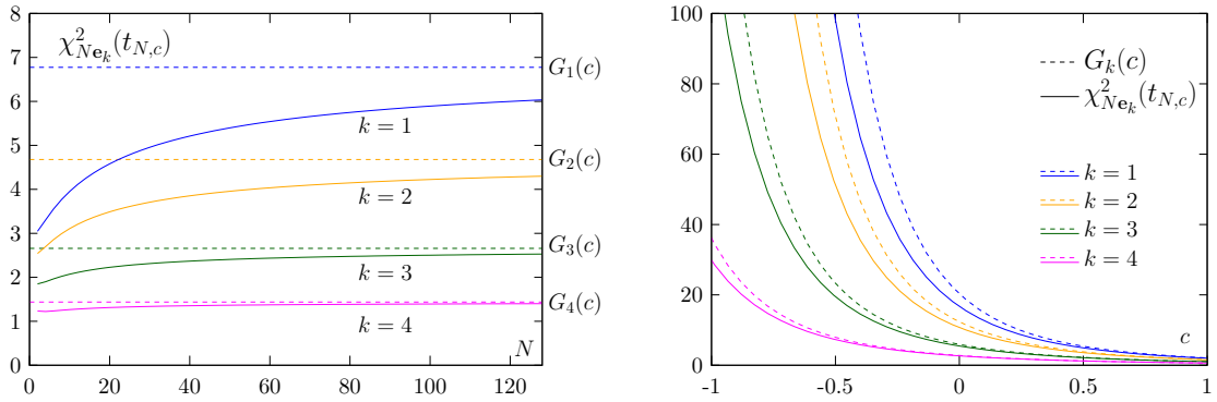
FIGURE 1. For parameters K = 4 , k \in [K] , \boldsymbol{\mu} = (0.7, 0.8, 1.0, 1.3) , p = 1.7 : left panel shows \chi_{N\mathbf{e}_k}^2(t_{N,c}) as a function of N , 2 \leq N \leq 128 for c = 0.4 , and right panel shows G_k(c) and \chi_{N\mathbf{e}_k}^2(t_{N,c}) as functions of c , with -1 \leq c \leq 1 , for N = 150 .
