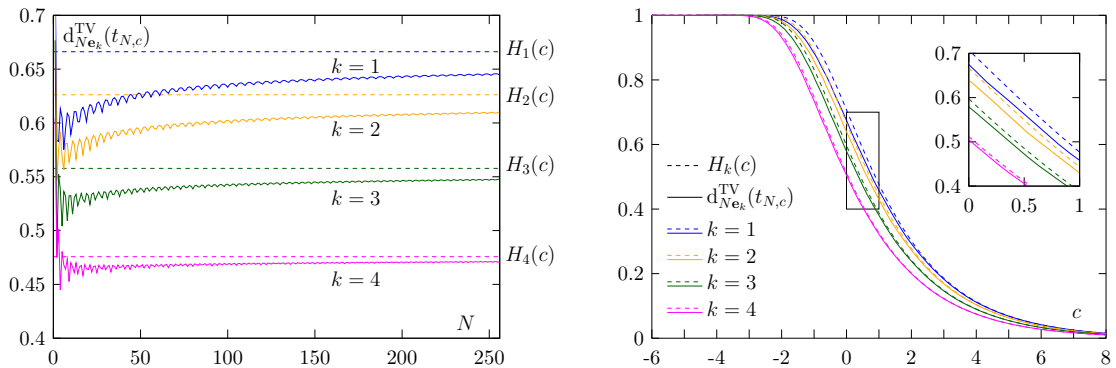
FIGURE 2. For parameters K = 4 , k \in [K] , \boldsymbol{\mu} = (0.7, 0.8, 1.0, 1.3) , p = 0 : left panel shows d_{N\mathbf{e}_k}^{\text{TV}}(t_{N,c}) as a function of N , 2 \leq N \leq 256 for c = 0.17 and right panel shows H_k(c) and d_{N\mathbf{e}_k}^{\text{TV}}(t_{N,c}) as functions of c , with -6 \leq c \leq 8 , for N = 100 .
