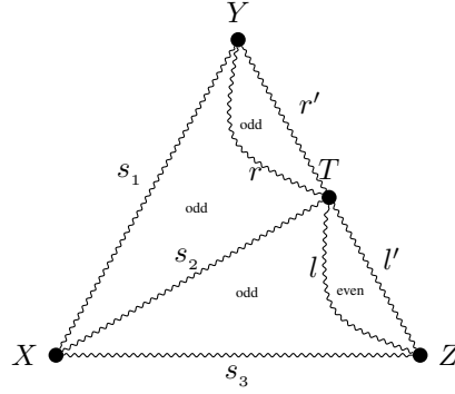
Figure 5: Subdivision of a C_{2k+1} -cycle with 3 chords
