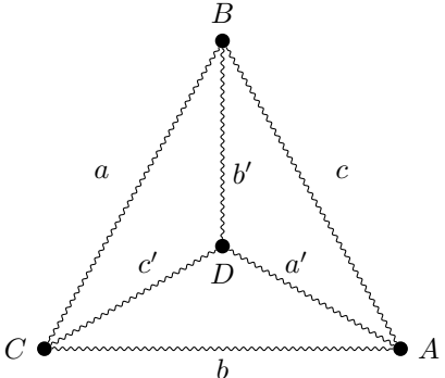
Figure 4: Labeling a K_4 -subdivision
