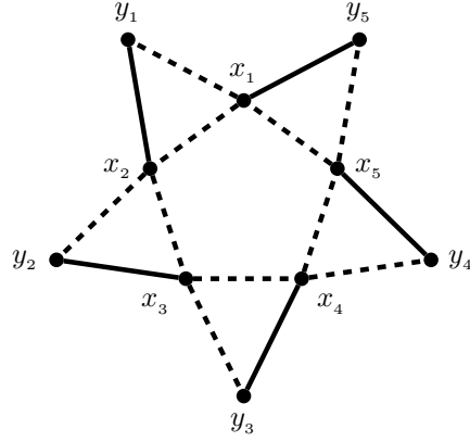
Figure 8: A signed K_4 -minor-free graph which does not map to \text{EDC}(SPal_5)
