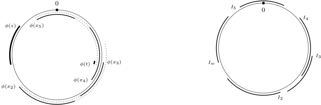
Figure 12: Case A-3: Updating ranges of \phi(x_i) 's Figure 13: Case A-3: Restrictions on wx_5x_4x_3x_2
