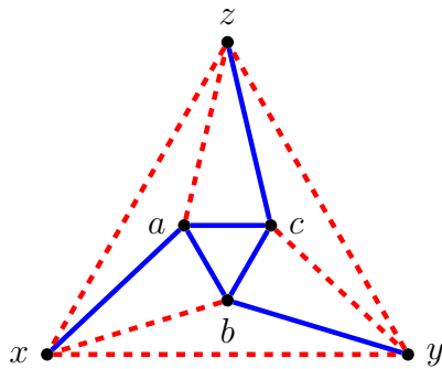
Figure 6: Mini-gadget (T, \pi)
