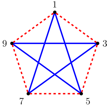
Figure 4: The signed Paley graph
