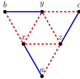
Figure 5: (F, \sigma)
