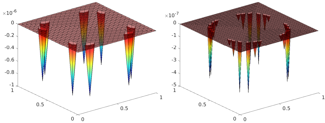
Figure 4: Negative part of the Lagrange multiplier for FEM \mathbb{P}_2 . Left: mesh \mathcal{T}_2 . Right: mesh \mathcal{T}_3 .
