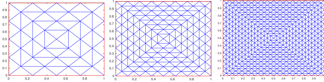
Figure 2: Left: coarse mesh \mathcal{T}_0 containing 64 elements with h_0 = 0.25 . Middle: first refined mesh \mathcal{T}_1 containing 256 elements with h_1 = 0.125 . Right: second refined mesh \mathcal{T}_2 containing 1024 elements with h_2 = 0.0625 .
