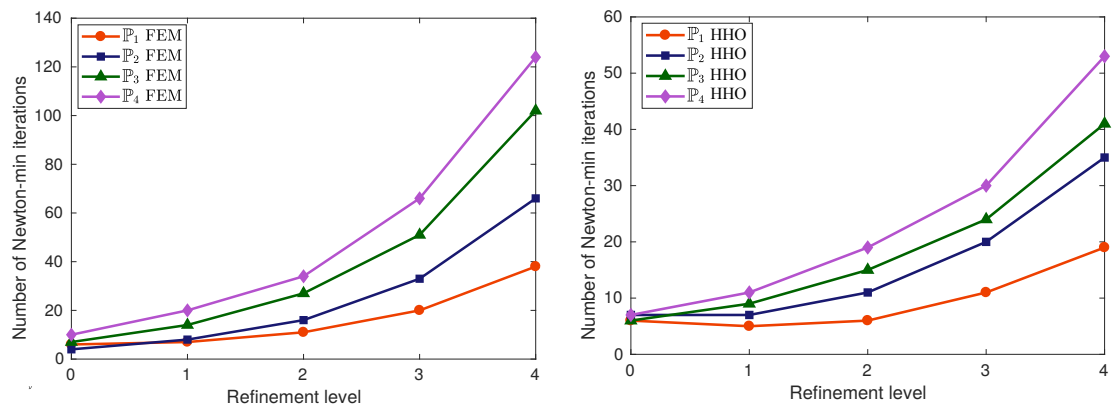
Figure 5: Number of Newton-min iterations for each refinement level. Left: FEM method. Right: HHO method.
