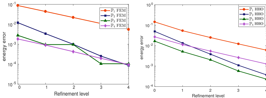
Figure 9: Energy norm error for each refinement level. Left: FEM method. Right: HHO method.
