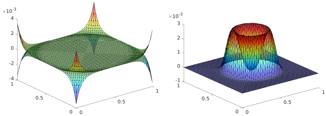
Figure 3: Solution at convergence for \mathbb{P}_2 FEM and mesh \mathcal{T}_3 . Left: position of the membranes (u_{1h}, u_{2h}) . Right: discrete Lagrange multiplier (\lambda_h) .
