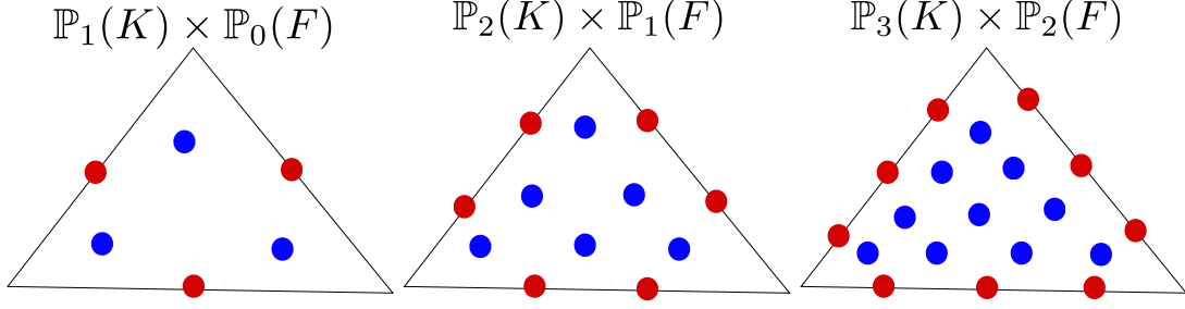
Figure 1: Representation of the degrees of freedom of \hat{U}_K . The cell DOFs are in blue, the edges DOFs are in red.
