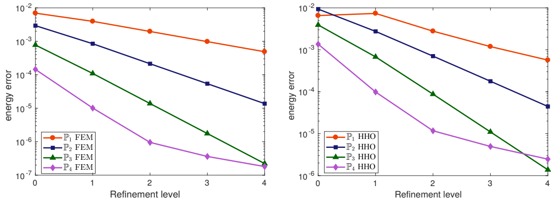
Figure 6: Energy norm error for each refinement level. Left: FEM method. Right: HHO method.
