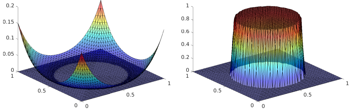
Figure 7: Solution at convergence for \mathbb{P}_2 FEM and mesh \mathcal{T}_3 . Left: position of the membranes ( u_{1h}, u_{2h} ). Right: discrete Lagrange multiplier ( \lambda_h ).
