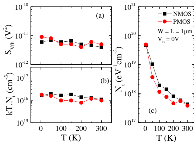
Fig. 9. S_{vib} (a), kT.N_t (b) and N_t (c) versus T for N- and PMOS. N_t = S_{vib} \cdot W \cdot L \cdot f \cdot C_{ox}^2 / q^2 \cdot \lambda \cdot kT , where \lambda is the tunneling constant in the dielectric.
