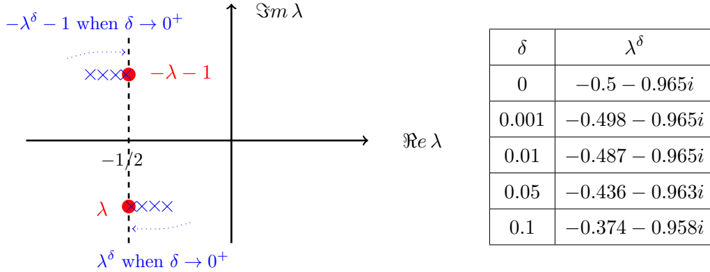
Figure 2: Behaviour of the eigenvalue \lambda^\delta close to the line \Re \lambda = -1/2 as the dissipation \delta tends to zero. Here the values have been obtained solving the problem (44) with a Finite Element Method. We work in the conical tip defined via (5) with \alpha = 2\pi/3 and \kappa_\varepsilon = -1.9 . In this case, using (6) we find I_\alpha \approx 2.585 so that the critical interval is approximately given by [-2.585; -1] .
