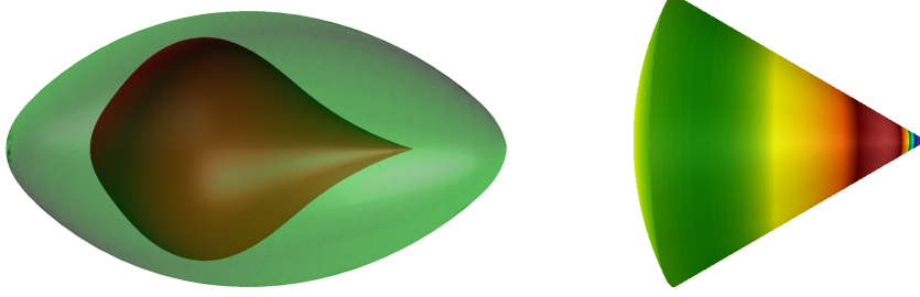
Figure 1: Left: the domain \Omega with the inclusion \mathcal{M} exhibiting a conical tip. Right: \mathfrak{s}|_{\mathcal{M}} for the circular conical tip with \alpha = \pi/6 (the critical interval is then approximately given by [-1; -0.1032] ) and \kappa_\varepsilon = -0.36 . In this situation, we have \eta \approx 2 .
