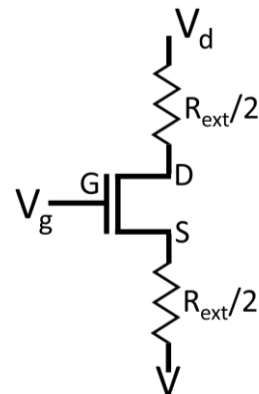
Fig. 1. Experimental set-up for monitoring the R_{SD} influence.
