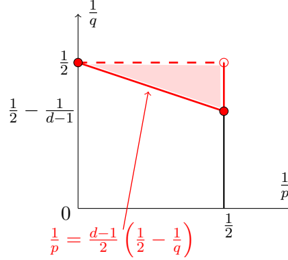
FIGURE 3. Admissibility in dimension d \geq 4 .
