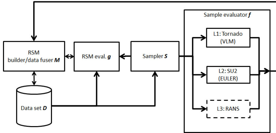
Figure 4: Workflow for data fusion in the MDA chain, interchangeable modules exchanging data using Brics.
