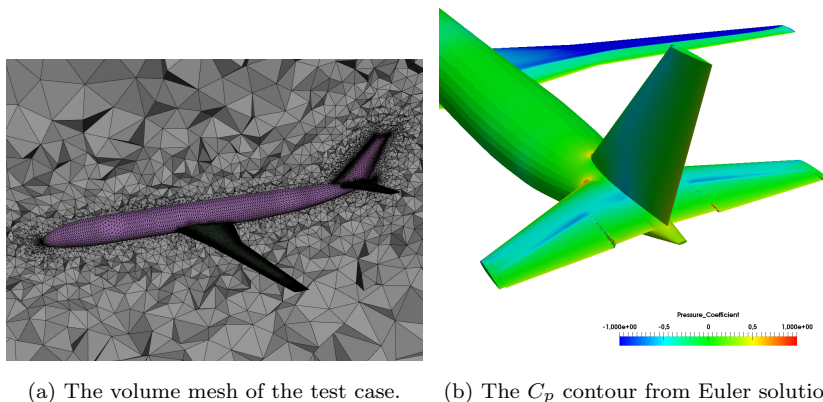
Figure 9: (a) The unstructured volume mesh with 5.9 million cells of the test case configuration, created by sumo [48] and TetGen [49]; (b) the C_p contour of the horizontal tail of the test case aircraft from Euler solutions computed by SU2, Mach=0.78, \alpha = 0^\circ with elevator deflection \delta = 4^\circ . The elevator deflection is modeled by deforming the mesh defining by FFD.
