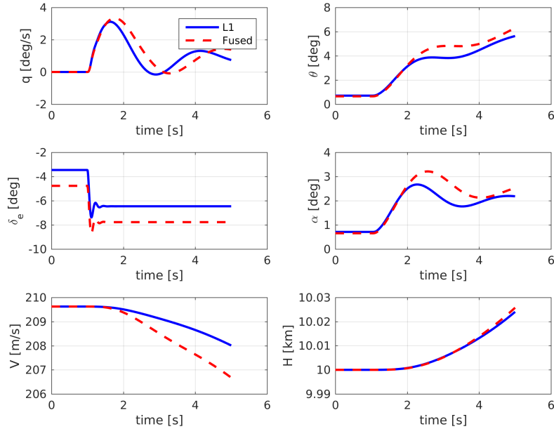
Figure 15: A step input on the elevator and its dynamic motion for a single Mach number M=0.7 .
