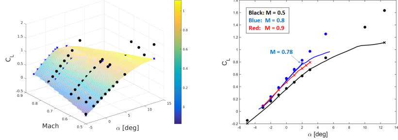
(a) Lift coefficient C_L surface and the sampled data. (b) Fused lift coefficient C_L for Mach number 0.5, 0.8 and 0.9.
