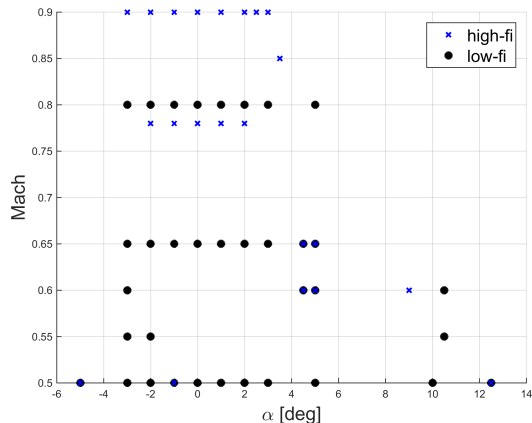
Figure 11: Final DOEs for building the surrogate models, viewed in a 2D space.
