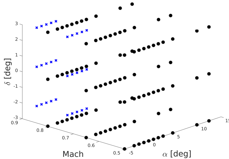
Figure 8: Initial DOE defined in the CPACS files. Black dot: low-fidelity data; blue cross: high-fidelity data.
