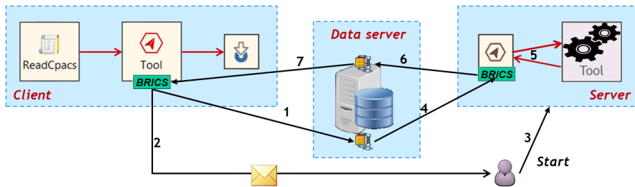
Figure 1: Schematic overview of Brics application in AGILE from within a client workflow and a server workflow, to accomplish remote tool execution [20].
