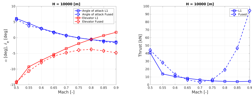
(a) Angle of Attack and elevator deflection. (b) The throttle setting.
