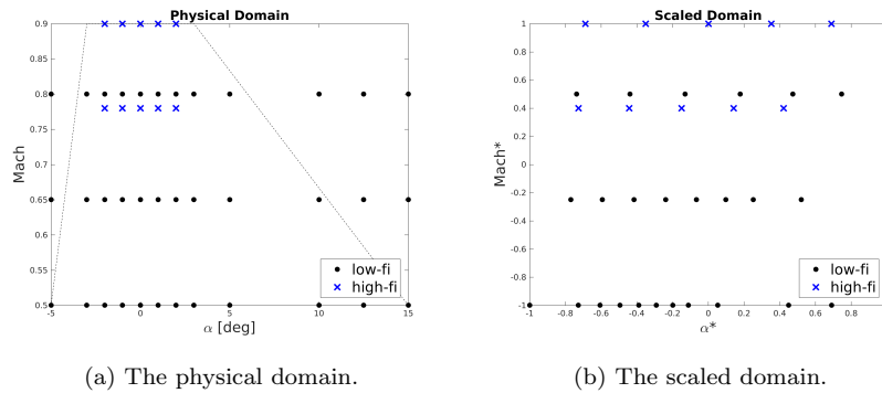
Figure 7: The initial samples of the domain for the Test Case and its transformation, at altitude 10 km.
