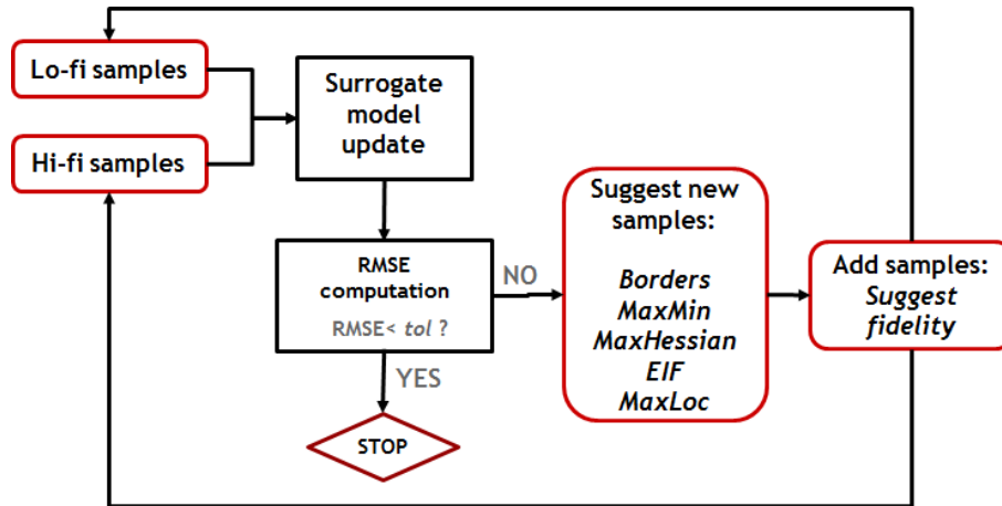
Figure 6: The "smart sampling" technology workflow.
