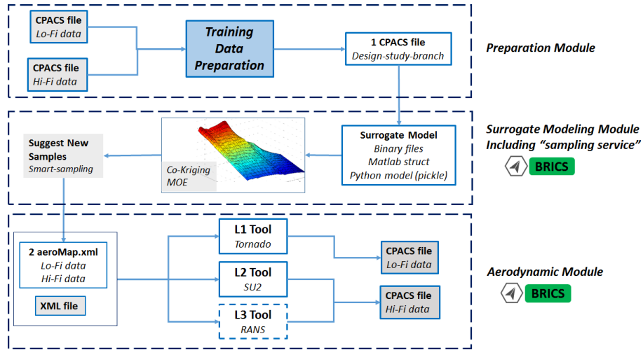
Figure 5: Data fusion service in the MDA chain with 3 stages.
