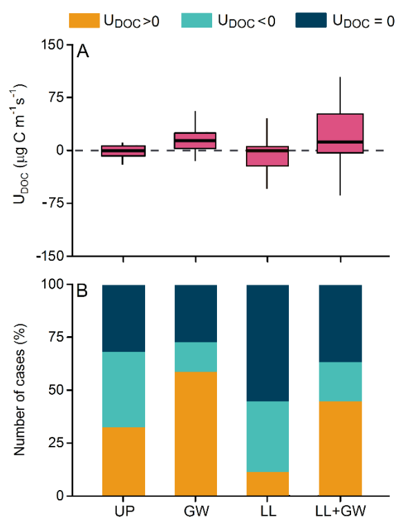
Figure 4. (A) In-stream net dissolved organic carbon uptake ( U_{\text{DOC}} ) for each scenario. Boxplots display the median, 25th, and 75th percentiles of U_{\text{DOC}} and whiskers extend to the 10th and 90th percentiles. The horizontal dashed line at U_{\text{DOC}} = 0 is shown as a reference. There were no differences among scenarios (Mann–Whitney test). (B) Relative number of cases when dissolved organic carbon (DOC) uptake prevailed over release ( U_{\text{DOC}} > 0 ), DOC release prevailed over uptake ( U_{\text{DOC}} < 0 ), and DOC uptake \sim DOC release ( U_{\text{DOC}} = 0 ) for each scenario. Differences in the proportion of U_{\text{DOC}} > 0 and U_{\text{DOC}} < 0 were only significant between scenarios GW and LL (Tukey’s test). Scenarios are: mostly upstream dissolved organic matter (DOM) inputs (UP), groundwater and upstream DOM inputs (GW), leaf litter and upstream DOM inputs (LL), and leaf litter, groundwater, and upstream DOM inputs (LL + GW).
