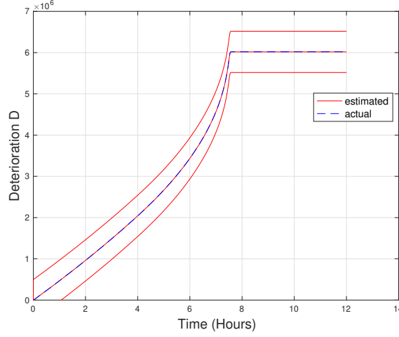
Figure 7: Estimation scenario: the deterioration level D and its uncertainty interval are estimated along the whole useful life of a given friction drive.
