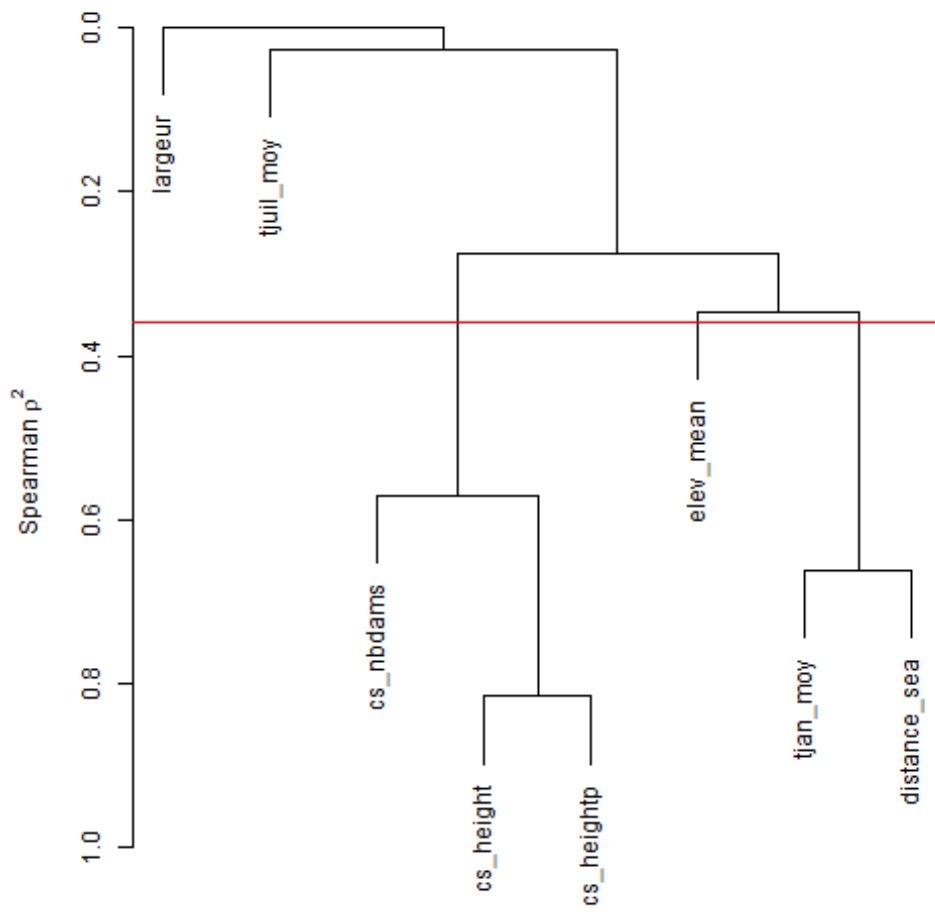
Figure 5.2 – Hierarchical clustering of the main continuous variables used in the model according to their collinearity.
