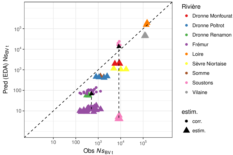
Figure 3.29 – Comparison of production estimated by EDA ( \widehat{N}_{s_{BV,t_a}} ), index river and fisheries estimated Silver eel run N_{s_{BV,t}} . \blacktriangle estimation of the total annual production, ( \bullet ) the EDA production has been raised by the surface of lakes and marshes which account for a large part of the water surface in this basin RHT.
