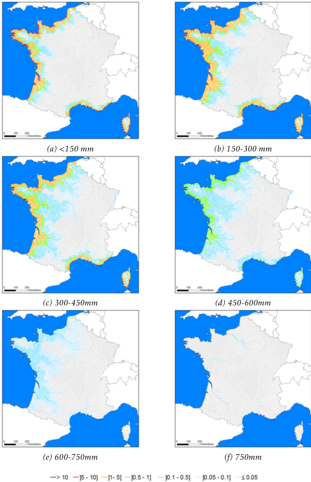
Figure 3.14 – Yellow eel densities (in eel.100 m -2 ) predicted per size class by the \Delta\Gamma model.
